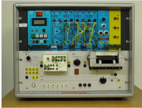
Small analog computer together with electromechanical servo. It is about 50 cm wide.
