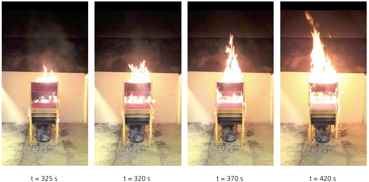
Figure 2.3. Different stages of the chair fire.
