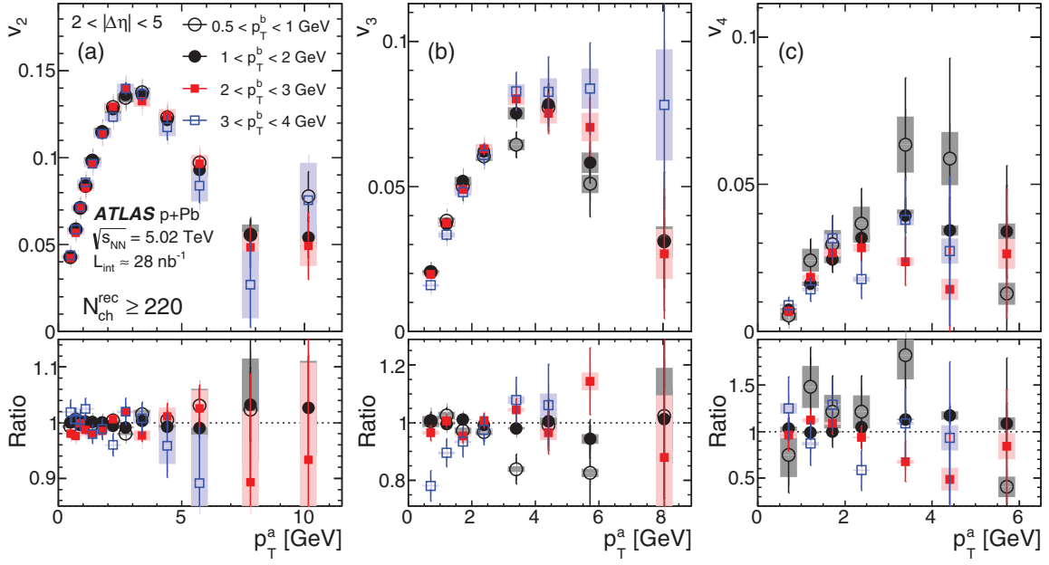
FIG. 10. (Color online) The v_2 (left column), v_3 (middle column), and v_4 (right column) as functions of p_T^a extracted using four p_T^b bins in the long-range region |\Delta\eta| > 2 for events with N_{ch}^{rec} \geq 220 . The ratio of the v_n(p_T^a) in each p_T^b bin to those obtained with the default reference p_T^b bin of 1–3 GeV are shown in the bottom part of each column. The error bars and shaded bands represent the statistical and systematic uncertainties, respectively.
