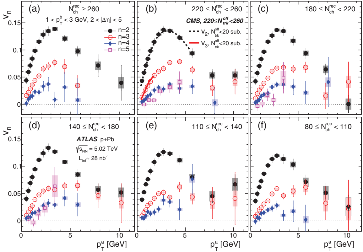
FIG. 9. (Color online) The v_n(p_T^a) with n = 2 to 5 for six N_{ch}^{rec} event-activity classes obtained for |\Delta\eta| > 2 and the p_T^b range of 1 – 3 GeV. The error bars and shaded boxes represent the statistical and systematic uncertainties, respectively. Results in 220 \leq N_{ch}^{rec} < 260 are compared to the CMS data [28] obtained by subtracting the peripheral events (the number of off-line tracks N_{trk}^{off} < 20 ), shown by the solid and dashed lines.
