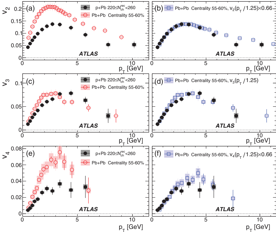
FIG. 16. (Color online) The coefficients v_2 (top row), v_3 (middle row), and v_4 (bottom row) as functions of p_T compared between p + Pb collisions with 220 \leq N_{ch}^{rec} < 260 in this analysis and Pb + Pb collisions in 55%–60% centrality from Ref. [9]. The left column shows the original data with their statistical (error bars) and systematic uncertainties (shaded boxes). In the right column, the same Pb + Pb data are rescaled horizontally by a constant factor of 1.25, and the v_2 and v_4 are also downscaled by an empirical factor of 0.66 to match the p + Pb data.
