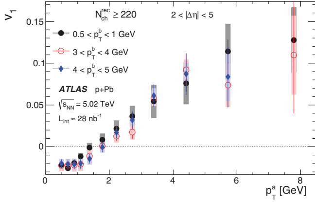
FIG. 15. (Color online) The p_T^a dependence of v_1 extracted using the factorization relations Eqs. (13) and (14) in three reference p_T^b ranges for events with N_{ch}^{rec} \geq 220 . The error bars and shaded boxes represent the statistical and systematic uncertainties, respectively.
