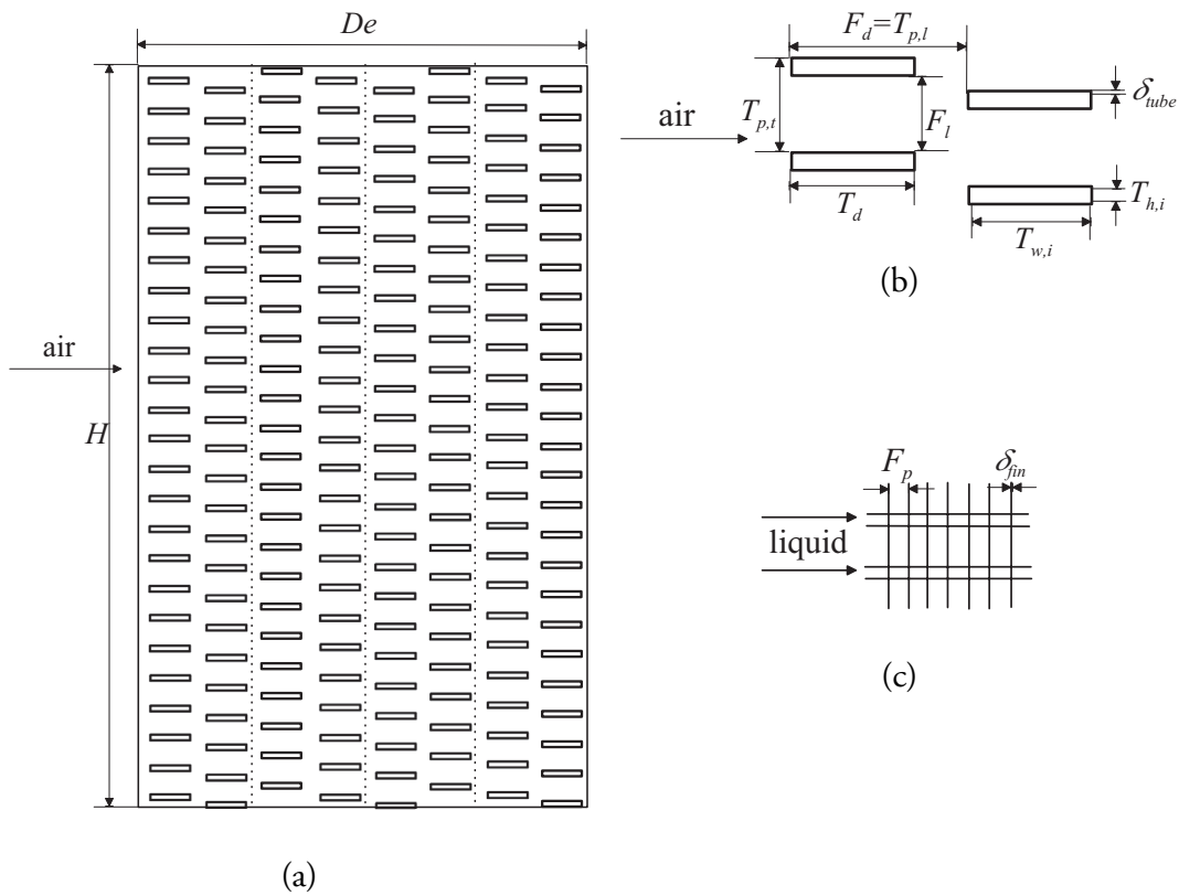
Figure 2.3. Schematic drawing and nomenclature of the “flat-fin-core” heat exchanger denoted FFC (Paper IV); (a) side view of cross-section, (b) enlargement of cross-section of staggered tube layout, (c) plate fin geometry, (c)
