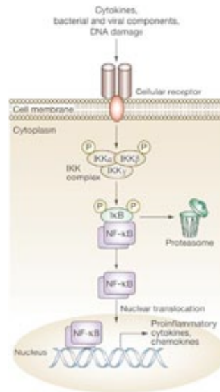
Figure9. Classical and atypical activating pathways of NF \kappa B.
