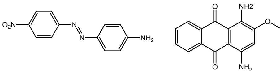
Figure 2. Examples of an azo dye (Disperse Orange 3) on the left and an anthraquinone (Disperse Red 11) on the right.
