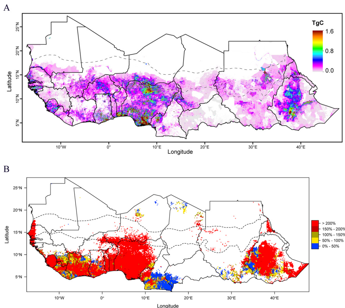
Figure 5. (A) Difference in NPP Demand over the region between 2000 and 2010 in areas that exhibited changes in population density of greater than one person per km 2 during the same time frame. (B) Percent of NPP Demand relative to NPP Supply between 2000–2010. Only areas with a statistical significance of p < 0.05 are shown here. Large areas, most notably in West Africa and Ethiopia, experience NPP Demand that is much larger than available supply.
