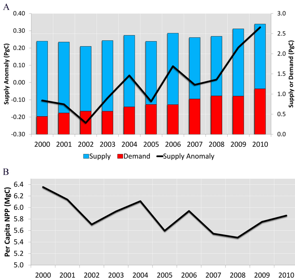
Figure 4. (A) Total NPP Supply , NPP Demand , and NPP Supply anomalies in the study area between 2000 and 2010. NPP Supply anomalies were computed as differences of NPP Supply from annual mean using the 11-year record. (B) Per capita NPP from 2000 to 2010. The total amount of NPP that is available to the region's population experienced abrupt declines in 2002 and 2005 (see section 3.1).
