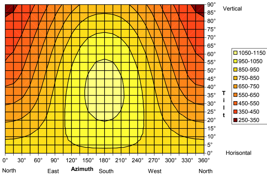
Figure 2.2 Global irradiation depending on different tilts and azimuth for the southern part of Sweden (Climate data for Jönköping average 1962-90) in \text{kWh/m}^2, \text{year} (Kjellsson 2000).
