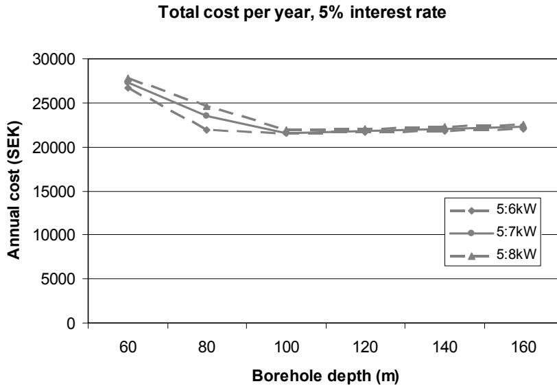
Figure 7.41 The total annual cost for the system 5 (recharging in winter and solar heated domestic hot water in summer) for the power of the heap pump 6, 7 and 8 kW_{th} respectively, with the cost of electricity 1 SEK/kWh, solar collector cost 7000 SEK/m interest rate 5%, 20 years lifetime and operation time, Stockholm climate for boreholes depths 60 – 160 m.
