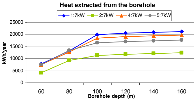
Figure 7.11 Heat extracted from the boreholes with the depths 60 – 160 m for four different systems. Reference case: Stockholm climate, heat pump power 7 kW th , 10 m 2 flat plate solar collector, about 29 400 kWh/year heat and DHW demand, result from operation year 20.
