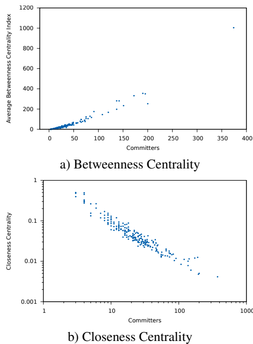
Figure 6: Centrality metrics over number of committers per project. Each data point represents one project
