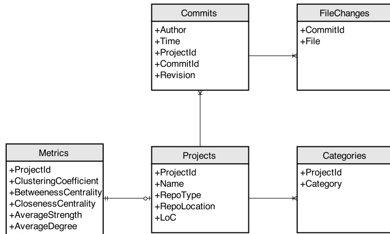
Figure 3: Database design
