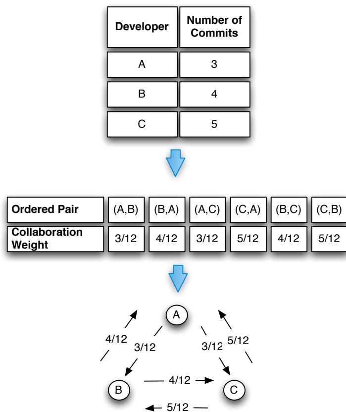
Figure 2: Transformation of the Extracted Data to the Weighted and Directed Pairs, Three Developers Changing the Same File Example
