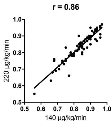
Figure 15. Unadjusted linear regression model: High dose adenosine showed a linear correlation to standard dose ( r = 0.86 , slope = 0.89).
