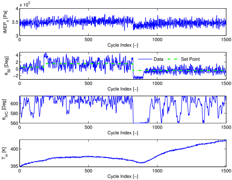
Figure 6.4 Experimental \text{IMEP}_n , \theta_{50} , and control signals \theta_{IVC} and T_{in} for the extended controller on the real engine.
