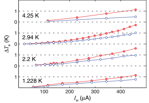
FIG. 2. (Color online) Measured source (red filled circles) \Delta T_{e,s} and drain (blue open circles) \Delta T_{e,d} electron temperature rises for T_0 = 1.228, 2.2, 2.94 , and 4.25 K. The relatively large temperature rise observed for the drain electrons, combined with the low electron conductance of the QD, indicates the presence of phonon-mediated heat flow into the drain-electron reservoir.
