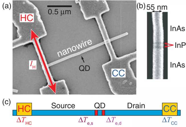
FIG. 1. (Color online) (a) A scanning electron micrograph (SEM) image of the HN system showing the hot (HC) and cold (CC) Au contacts, and the approximate position of the quantum dot (QD), not visible here. A temperature gradient is applied using an ac heating current I_H through the HC. (b) Closeup SEM image of the two InP barriers within the InAs nanowire. (c) Cross section of the nanowire and contacts along the nanowire axis. \Delta T_{(HC,CC)} are the heating-induced electron temperature rises above the background temperature T_0 in the hot and cold contacts, respectively. \Delta T_{e,(s,d)} are the source and drain-electron temperature rises measured in the vicinity of the quantum dot. The source and drain portions of the NW are defined by the direction of heat flow, the source being closest to the HC.
