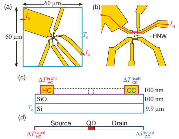
FIG. 3. (Color online) (a), (b) Top- and (c) side-view schematics of the simulated area for the Au leads and substrate, called the substrate simulations in the text. The location of where the HN would be is shown by dashed lines in panels (b) and (c). The outer boundary in (a) and lower boundaries in (c) (blue lines) are set to the background temperature T_0 . The top boundary in (c) (purple line) is assumed to be a perfect insulator. The red line in panel (b) shows the path of the heating current I_H . Panel (d) shows a schematic of the simulated HN. In panels (c) and (d), \Delta T_{HC}^{(e,ph)} and \Delta T_{CC}^{(e,ph)} represent the electron and phonon temperature rises in the HC and CC, respectively, as well as the boundary conditions for the simulated HN.
