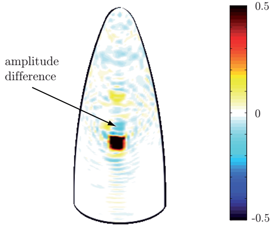
Figure 15: The difference (|E_{\text{radome}}^v| - |E_{\text{def radome}}^v|) / \max||E_{\text{radome}}^v| - |E_{\text{def radome}}^v|| in a linear scale on the front side of the radome. The scale is truncated in order to see the small field amplitude above the copper plate, marked with an arrow.
