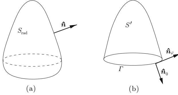
Figure 22: (a) The surface S_{\text{rad}} and its outward unit vector \hat{\mathbf{n}} . (b) The surface S' bounded by the curve \Gamma . The unit normal vectors are; \hat{\mathbf{n}}_\varphi - tangent to \Gamma and S' , \hat{\mathbf{n}}_0 tangent to S' and normal to \Gamma . That is \hat{\mathbf{n}}_0 = \hat{\mathbf{n}}_\varphi \times \hat{\mathbf{n}} .
