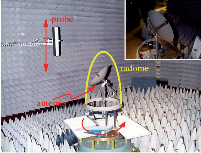
Figure 1: Photo of the cylindrical near-field range at SAAB Bofors Dynamics, Sweden. The antenna under test is rotated and the probe is moved in the vertical direction. A close up of the reflector antenna is shown in the upper right corner.
