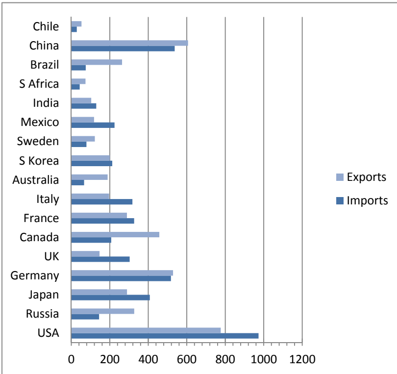
Figure 6.1. Ecological footprints of trade 2006, million global hectares My calculation. Data courtesy Global footprint network. The countries included are the 13 major trading nations and the most recent members of the OECD (Chile, Mexico, and South Korea) plus Sweden.
