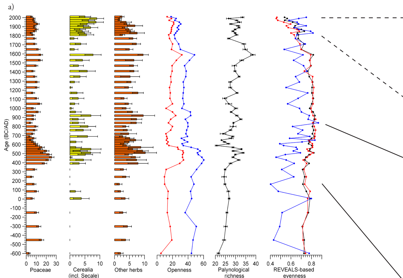
Figure 7. Quantitative estimates of regional vegetation cover for selected taxa/taxa groups, openness, palynological richness and REVEALS-based evenness based on pollen counts from Lake Fiolen, for a) the entire sequence studied 600 BC-AD 2008, b) the last 200 years, and c) the period AD 200-900. The dashed lines illustrate that a different chronology was used for b), making the records not directly comparable. Openness includes all herbs (red line) and all herbs including Corylus and Juniperus (blue line). REVEALS-based evenness was calculated for 26 taxa (black line), but also for trees (red line) and herbs (blue line) separately. Regional rural population data for the last 200 years is also shown. The sequence was divided into different land-use periods described in detail in Appendix I and II.
