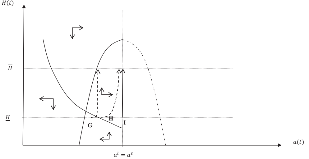
Figure 5. Illustration of the shape of the stationary loci, and trajectories for the truncated vertical terminal line problem, the case when a^l = a^s . The \frac{dH}{dt} = 0 locus is a parabola with an inflexion point at a(t) = a^l , and intersections with the a -axis at a(t) = a^l \pm \sqrt{\frac{TE^l}{\varphi^l}} . The \frac{da}{dt} = 0 loci is a hyperbola, with the vertex at a(t) = a^s . The equilibrium (at the intersection of the parabola and the vertical line) is locally stable.
