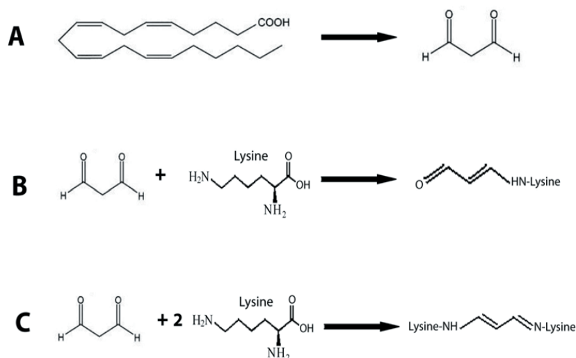
Figure 3: (A) The formation of MDA during the breakdown of fatty acid. (B) The formation of MDA adducts on lysine. (C) MDA induced cross linking.
