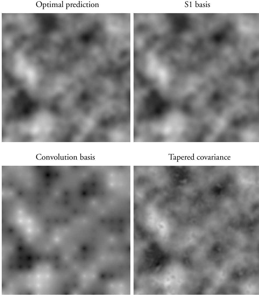
Figure 5: An example of an optimal kriging prediction and predictions using the S1 basis, the convolution basis, and a tapered covariance when \nu = 2 and the covariance range is 1. The predictions are based on 5000 observations and are calculated for a 200 \times 200 grid in the square [0, 5] \times [0, 5] . The number of basis functions and the tapering range are chosen such that the total time for Step 2 and Step 3 is approximately equal for the different methods.
