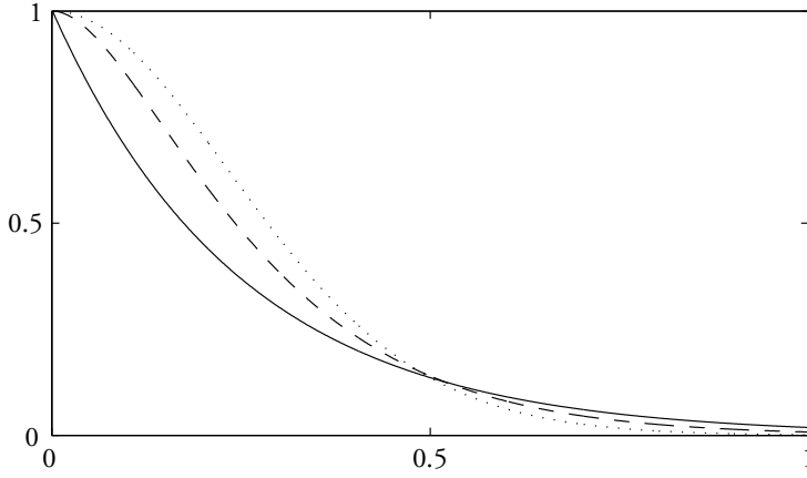
Figure 1: Matérn correlation functions shown for \nu = 0.5 (solid line), \nu = 1.5 (dashed line), and \nu = 10 (dotted line), with \kappa = \sqrt{8\nu}/0.5 .
