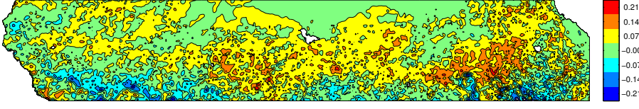
Figure 6: Contour plot of the GMRF estimate of the \mathbf{K}_2 field. Here, colours corresponding to positive values correspond to areas with a positive linear increase in vegetation. Notice that a large number of these areas coincides with areas with significant positive trends in Figure 5. Also observe that this figure has a different colour scale than Figure 4.
