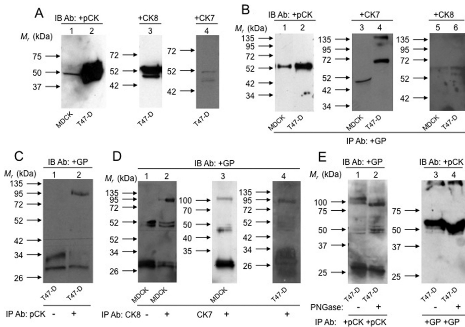
Fig. 7. Native GP1R-CK association. A, MDCK cells (MDCK, lane 1) and T47-D cells (T47-D, lanes 2–4) were lysed and immunoblotted with mouse pan-CK antibody (lanes 1 and 2), mouse CK8 antibody (lane 3), or mouse CK7 antibody (lane 4). B, MDCK cells (MDCK, lanes 1, 3, and 5) and T47-D cells (T47-D, lanes 2, 4, and 6) were lysed, immunoprecipitated with goat GP1R antibody (GP) precoupled to protein G-Sepharose, and then immunoblotted with pan-CK antibody (lanes 1 and 2), CK7 antibody (lanes 3 and 4) or CK8 antibody (lanes 5 and 6). C, T47-D cells (T47-D) were lysed, immunoprecipitated with protein G-Sepharose without (–, lane) and with precoupled pan-CK antibody (+, lane), and then immunoblotted with GP1R antibody (GP). D, MDCK cells (MDCK, lanes 1–3) and T47-D cells (T47-D, lane 4) were lysed, immunoprecipitated with CK8 antibody (lanes 1 and 2) or CK7 antibody (lanes 3 and 4) precoupled to protein G-Sepharose, and then immunoblotted with GP1R antibody. E, T47-D cells (T47-D) were lysed, immunoprecipitated with pan-CK antibody (lanes 1 and 2) or GP1R antibody (lanes 3 and 4) precoupled to protein G-Sepharose, respectively, treated without (lanes 1 and 3) or with PNGase F (lanes 2 and 4) and then immunoblotted with GP1R antibody. Molecular mass ( M_r ) standards (in kilodaltons) (left side arrows) are indicated. The results are representative of experiments performed at least three times.
