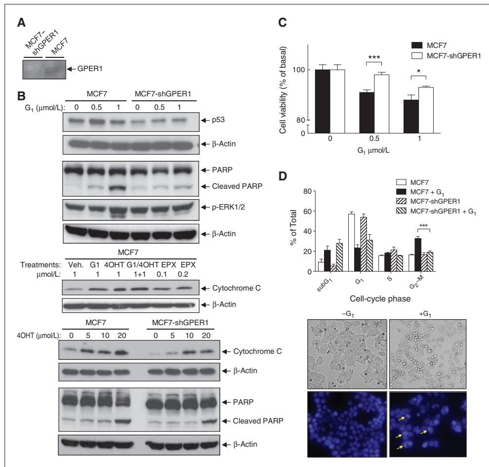
Figure 3. Constitutive and agonist-stimulated proapoptotic GPER1 signaling in MCF7 cells. A, immunoblotting of GPER1 in MCF7 cells without (MCF7) and with GPER1 shRNA knockdown (MCF7-shGPER1). B, immunoblotting of p53, cleaved PARP, phosphorylated ERK1/2 (p-ERK1/2), and cytochrome C release in MCF7 cells without (MCF7) and with GPER1 shRNA knockdown (MCF7-shGPER1) and treated with different concentrations of G 1 (G 1 ), 4OHT, and EPX for 24 hours as indicated. β-Actin serves as a loading control. C, viability of MCF7 cells without (MCF7) and with GPER1 shRNA knockdown (MCF7-shGPER1) and treated without and with increasing concentrations of G 1 for 24 hours as determined with the MTT assay. D, cell-cycle phases in MCF7 cells without (MCF7) and with GPER1 shRNA knockdown (MCF7-shGPER1) and treated without and with 1 μmol/L G 1 for 24 hours as determined by flow cytometry, and morphologic changes and chromatin condensation/nuclear fragmentation as determined by Hoechst 33342 staining in MCF7 cells following treatment without (-G 1 ) and with 1 μmol/L G 1 (+G 1 ) for 24 hours. Yellow arrows indicate fragmented nuclei. *, P < 0.05 ; ***, P < 0.001 .
