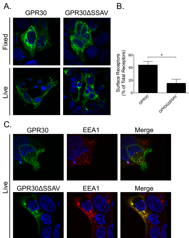
FIGURE 3. GPR30 requires the C-terminal PDZ motif for plasma membrane retention. A, HEK cells transfected with GPR30 or GPR30 \Delta SSAV were subjected to fixed staining (Fixed) and live staining (Live) with M1 FLAG antibodies. B, HEK cells transfected with GPR30 or GPR30 \Delta SSAV were stained live (Surface Receptors) and following permeabilization (Total Receptors) with M1 FLAG antibodies and then subjected to flow cytometry. The values are means \pm S.E. of at least three independent experiments with each data point performed in at least triplicates. C, HEK cells transfected with GPR30 or GPR30 \Delta SSAV were subjected to live staining with M1 FLAG antibodies. Following fixation and permeabilization, cells were stained with EEA1 antibodies. A and C, the results are representative of experiments performed at least three times. The individual and merged images (Merge) were collected using a Nikon Eclipse confocal microscope, \times 60 objective, and 50- \mu m zoom. Yellow indicates colocalization in merged images. *, p < 0.05 .
