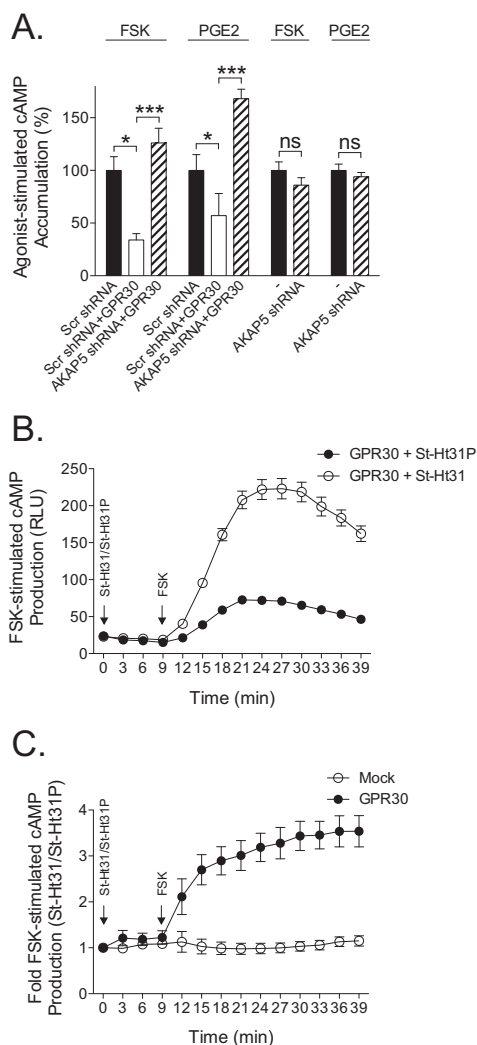
FIGURE 7. AKAP-RIL mediates GPR30 inhibition of cAMP production. A , HEK cells were transfected by nucleofection without or with GPR30, scrambled (Scr) shRNA, or AKAP5 shRNA. After 48 h, cells were stimulated with 1 \mu M FSK for 30 min and, after 96 h, with 1 \mu M PGE 2 for 30 min. cAMP was measured with RIA, and the values are mean \pm S.E. of at least three independent experiments, with each data point representing 3–16 measurements. * p < 0.05; *** p < 0.001. B , HEK cells were transfected with GPR30 and treated with 50 \mu M St-Ht31 or St-Ht31P and 1 \mu M FSK. The result, shown as relative light units (RLU), is representative of three experiments, with each data point being the mean \pm S.E. of 24 measurements. C , HEK cells were transfected without (Mock) and with GPR30 and treated with 50 \mu M St-Ht31 or St-Ht31P and 10 \mu M FSK. B and C , cAMP was measured in real time with the GloSensor assay. The effect of St-Ht31 was determined, i.e. each measurement was normalized to basal (time = 0 min), and each data point was the mean \pm S.E. of 24 measurements, with measurements including St-Ht31 normalized to those including St-Ht31P.
