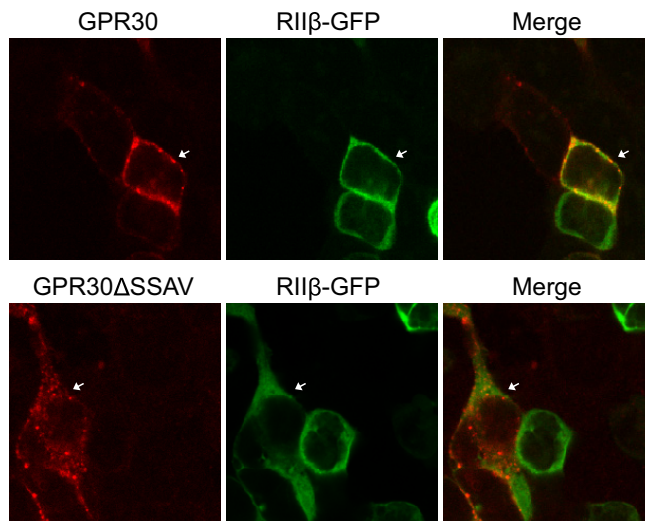
FIGURE 6. The GPR30-MAGUK-AKAP5 complex is colocalized with the PKA RII \beta regulatory subunit in the plasma membrane. HEK cells transfected with PKA RII \beta -GFP (RII \beta -GFP) together with GPR30 or GPR30 \Delta SSAV were subjected to live staining with M1 FLAG antibodies. The results are representative of experiments performed at least three times. The individual and merged images (Merge) were collected using a Nikon Eclipse confocal microscope, \times 60 objective, and 50- \mu m zoom. The arrows indicate cells coexpressing PKA RII \beta -GFP either with GPR30 or GPR30 \Delta SSAV.
