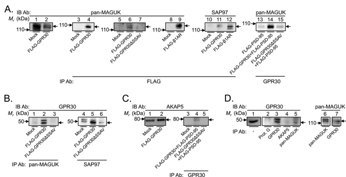
FIGURE 4. The GPR30 C-terminal PDZ motif forms a complex with MAGUKs and AKAP5. A , lysates of naïve HEK cells (Mock, lane 1) and HEK cells stably expressing mouse GPR30 (FLAG-GPR30, lane 2) were immunoblotted (IB) with pan-MAGUK antibody or first immunoprecipitated (IP) with M2 FLAG Ab beads and then IB with pan-MAGUK Ab (lanes 3 and 4). Lysates of HEK cells transfected without (Mock, lanes 5, 8, and 10) and with human GPR30 (lanes 6 and 11), GPR30 \Delta SSAV (lane 7), or \beta 1-AR (lanes 9 and 12) were immunoprecipitated with M2 FLAG Ab beads and then immunoblotted with pan MAGUK Ab (lanes 5–9) or SAP97 Ab (lanes 10–12). Lysates of HEK cells transfected with PSD-95 without (lane 13) and with human GPR30 (lane 14) or GPR30 \Delta SSAV (lane 15) were immunoprecipitated with GPR30 Ab-protein G beads and then immunoblotted with pan-MAGUK Ab. B , lysates of HEK cells transfected without (lane 1) and with GPR30 (lane 2) or GPR30 \Delta SSAV (lane 3) were immunoprecipitated with pan-MAGUK Ab-protein G beads and then immunoblotted with GPR30 Ab. C , lysates of naïve HEK cells (lane 1) and HEK cells stably expressing mouse GPR30 (lane 2) were immunoblotted with AKAP5 antibody. Lysates of HEK cells transfected with PSD-95 without (lane 3) and with human GPR30 (lane 4) or GPR30 \Delta SSAV (lane 5) were immunoprecipitated with M2 FLAG Ab beads and then immunoblotted with AKAP5 antibody. D , lysates of MDCK cells were immunoblotted with GPR30 antibody (lane 1) or first immunoprecipitated with protein G beads (lanes 2) or protein G beads bound with GPR30 Ab (lanes 3 and 7), AKAP5 Ab (lane 4), or pan-MAGUK Ab (lanes 5 and 6) and then immunoblotted with GPR30 Ab (lanes 2–5) or pan-MAGUK Ab (lanes 6 and 7). Molecular weight ( M_r ) standards (in kilodaltons) are indicated (arrows on the left). MAGUKs ( A and D , lanes 6 and 7), GPR30 ( B and D , lanes 1–5), and AKAP5 ( C ) are indicated (arrows on the right). The results are representative of experiments performed at least three times.
