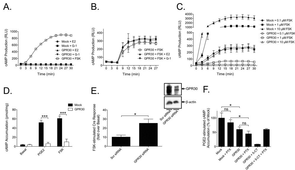
FIGURE 1. GPR30 constitutively inhibits cAMP production. A and B, HEK cells transfected without (Mock) and with GPR30 were treated with 0.1 μM E 2 , 1 μM G-1, and/or 1 μM FSK. C, HEK cells transfected without and with GPR30 were treated with increasing concentrations of FSK. D, CHO cells transfected without and with GPR30 were treated with 1 μM PGE 2 or 1 μM FSK for 30 min. E, MDCK-Cre cells transfected with scrambled (Scr siRNA) and GPR30-specific siRNA (GPR30 siRNA) were treated with 1 μM FSK and immunoblotted for GPR30 and β-actin. F, CHO cells transfected without and with GPR30 were treated without and with 100 ng/ml pertussis toxin (PTX) for 24 h and then with 1 μM PGE 2 without or with 100 nM 5-carboxamidotryptamine (5-CT) for 30 min. A–C, cAMP was measured in real time with the GloSensor assay, and the results, shown as relative light units (RLU), are representative of at least six experiments, with each data point being the mean ± S.E. of 8–16 measurements. In D and F, cAMP was measured with RIA, and in E, cAMP was measured with the Cre reporter assay, and the values are means ± S.E. of at least three independent experiments, with each data point representing 3–16 measurements. *, p < 0.05 ; ***, p < 0.001 ; ns, not significant.
