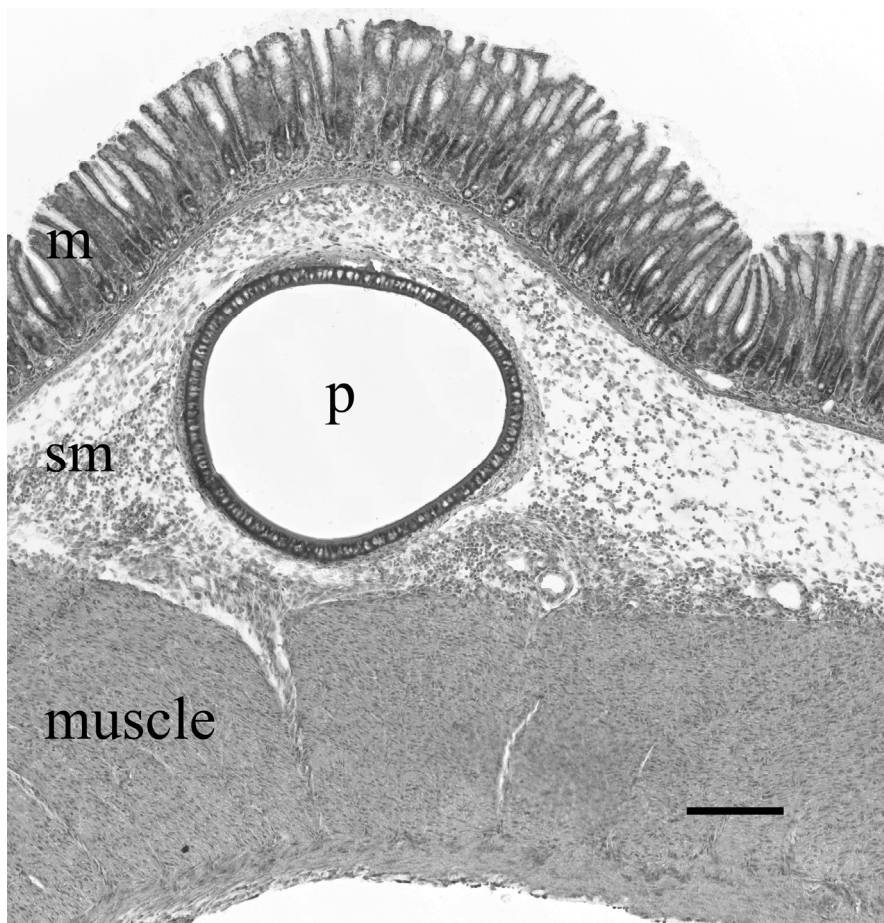
Fig. 5. Transverse section (12μm thick) of the antral wall (stained with haematoxylin and erythrosin), showing mucosa (m), microdialysis probe (p) in the submucosa (sm), and muscularis externa (muscle). Bar = 200 μm. The probe resembles a large blood vessel.
