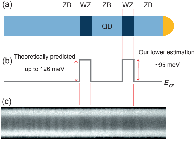
Figure 2.1: (a) Schematic illustration of a quantum dot defined by wurtzite segments in an otherwise zinc blende InAs nanowire. (b) Sketched conduction-band ( E_{CB} ) alignment of the corresponding system, where the wurtzite segments are assumed to form square potential barriers in the conduction band. (c) SEM image of a crystal phase-defined quantum dot; using information from TEM images on the structural composition of typical nanowires from the same growth substrate, the wurtzite segments can be distinguished in the contrast profile, see Section 2.6.
