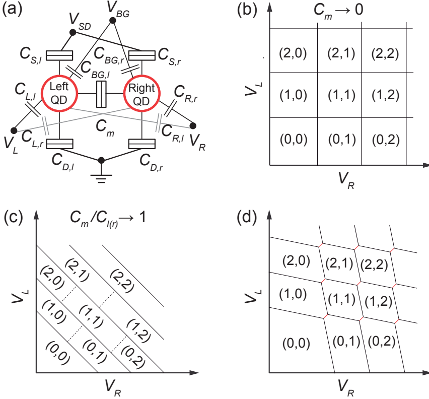
Figure 4.2: (a) Network of resistors and capacitors representing the two parallel-coupled quantum dots in the constant interaction model. Tunnel barriers connect both dots to the source and drain. The dots are capacitively coupled to three gates. (b)-(d) Charge stability diagrams showing the charge transition borders as a function of the two side gates for: (b) a decoupled double quantum dot, (c) a fully capacitively coupled double quantum dot (single dot) and (d) an intermediate capacitively coupled double quantum dot (honeycomb diagram). The equilibrium electron numbers ( N_l, N_r ) are indicated.
