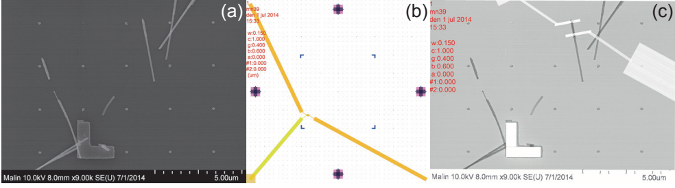
Figure 2.8: (a) Low-resolution SEM image of a nanowire selected for contact processing. (b) Visualization of the design file used in the EBL exposure. (c) The original SEM image with the design file superimposed. The L-shaped structure is a part of the coordinate system on the measurement substrates that enables alignment of the contacts.
