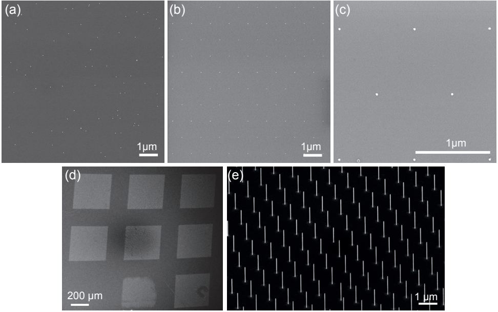
Figure 2.6: SEM images: (a) Au aerosol particles with a diameter of 39 (\pm 5.5) nm and an areal density of 0.87 \mu\text{m}^{-2} (Image contribution: Robert Hallberg). (b) and (c) Low and high resolution images of EBL-defined Au particles with a 1 \mu\text{m} pitch and a diameter of approximately 25 nm. For exposure, VOYAGER High speed EBL from Raith with 50 kV acceleration voltage and 3 fC dose was used. (d) Overview image of a sample after nanowire growth with square fields with different particle sizes. (e) A zoomed-in view of nanowire arrays.
