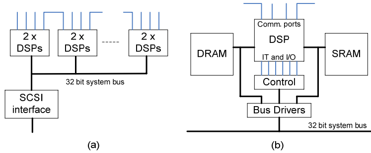
Figure 3.1 The architecture of the ACE board (a) and a single DSP with corresponding storage and control units (b).
