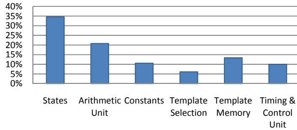
Figure 3.8 The amount of allocated logic for each of the blocks relative to the entire size of a single PE. Putting together the bars representing state values, constant values and template selection gives the total area of register arrays.
