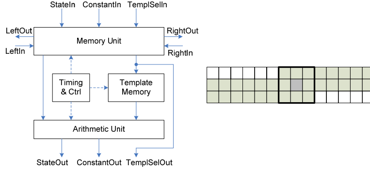
Figure 3.6 Left: a schematic view of the processing unit in CASTLE, where dashed lines represent control signals and continuous lines shows data path. Right: the belt of pixels stored on chip for 1-neighborhood where the black square indicates the current position of the convolution operation.
