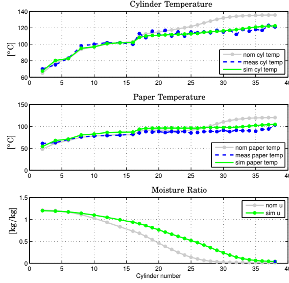
Figure 6 Stationary temperature and moisture profiles. The x-axis shows cylinder numbers.
