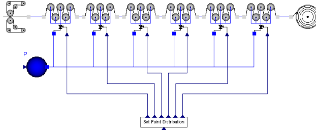
Figure 5 The top level of a complete dryer section model.
