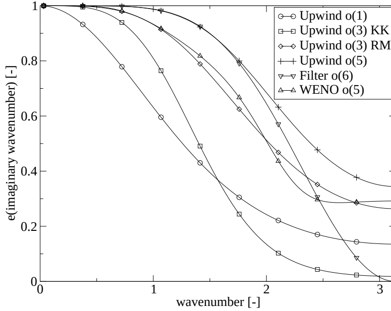
Figure 5.6: Dissipation error
