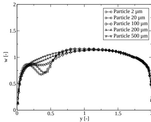
e) Streamwise flow profiles for various particle injection diameters
