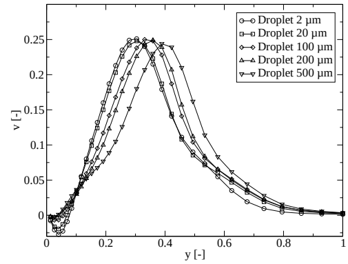
d) Cross-stream flow profiles for various droplet diameters
