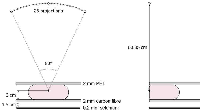
Figure 13. Geometry of the modelled BT system. The centre of rotation is placed at the chest wall side 60.85 cm below the X-ray source and 3 cm above the support plate.
