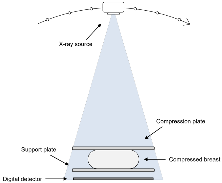
Figure 6. In BT, the X-ray source moves over a limited angular range while projection images of the breast are acquired by the detector. The breast is compressed between the support and compression plate to immobilize it, reducing motion artefacts, separate structures in the breast, which is especially important in 2D DM, and reduce and equalize the breast thickness, which reduces the effects of scattered radiation, reduces the radiation dose, and enhances the image contrast (Perry et al. 2008).
