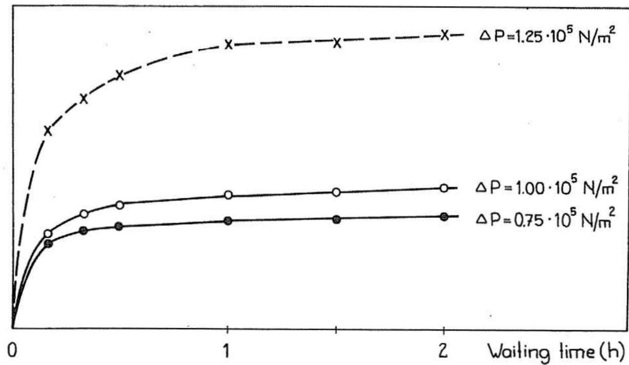
FIG 20 Effect on permeability of waiting-time at water-air displacement. Clay brick, size 30 \text{ cm}^2 , thickness 30 \text{ mm} .
