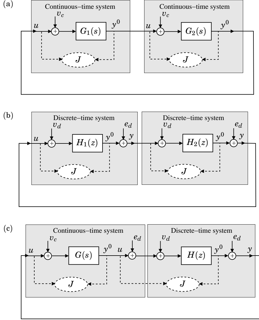
Figure 2 Possible interconnections of continuous-time and discrete-time systems.
