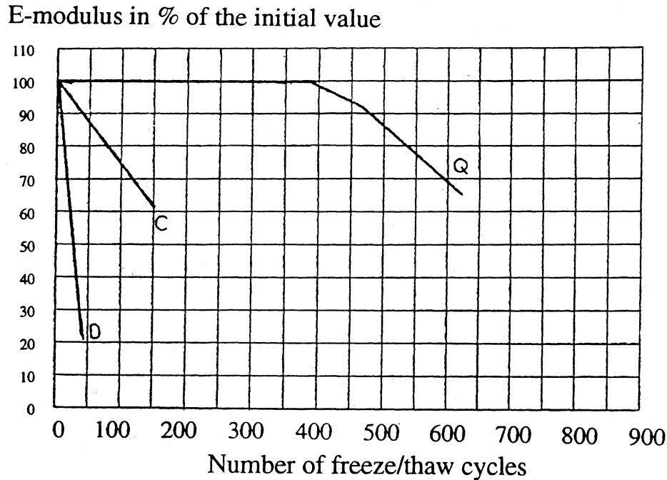
Fig 13: The damage as function of the number of freeze/thaw cycles at unisolated freeze/thaw testing of three cement mortars; /11/.
