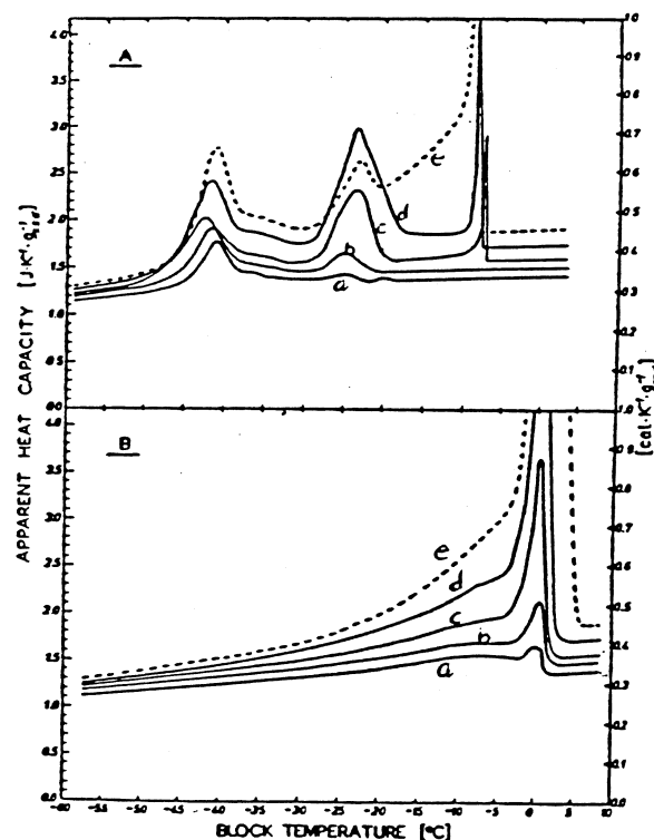
Fig 20: Calorimeter measurements of never-dried cement pastes with different water/cement ratio; /15/. A: Cooling phase. B: Thawing phase. (a. w/c=0,35 ; b. w/c=0,40 ; c. w/c=0,45 ; d. w/c=0,50 ; e. w/c=0,60 ).
