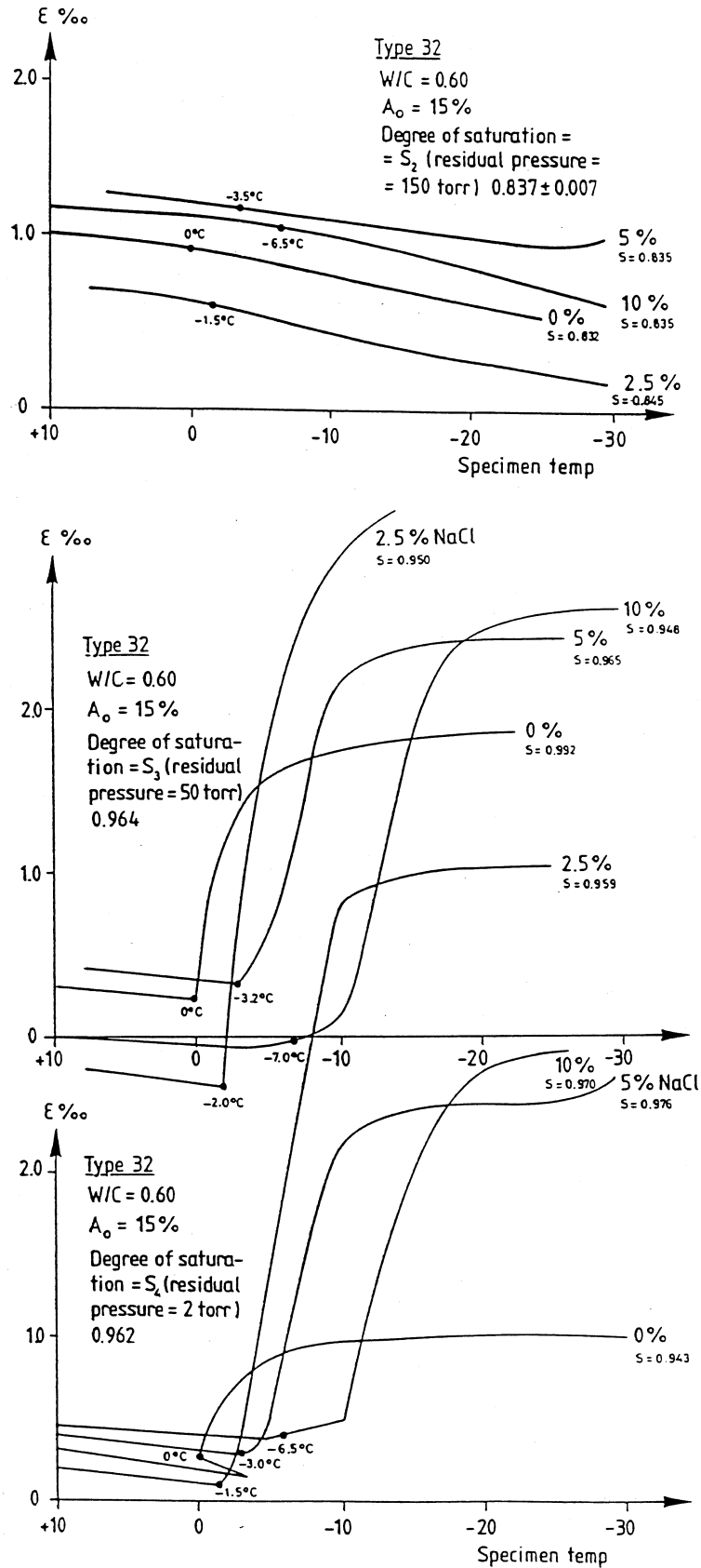
Fig 23: Length change versus temperature during freezing of cement mortar with w/c=0.60 , vacuum-saturated at different residual pressures and containing salt solutions of different concentration; /19/.
