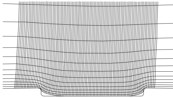
Figure 13: Element deformation when running over a small groove using an elastoplastic finite element model.
