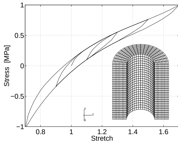
Figure 16: Amplitude dependent dynamic stiffness. Analysis of a cylindric component subjected to axial cyclic tensile/compressive load.
