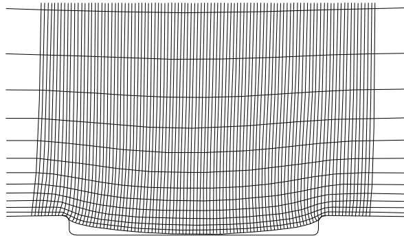
Figure 11: Element deformation when running over a small groove using an elastic finite element model.
