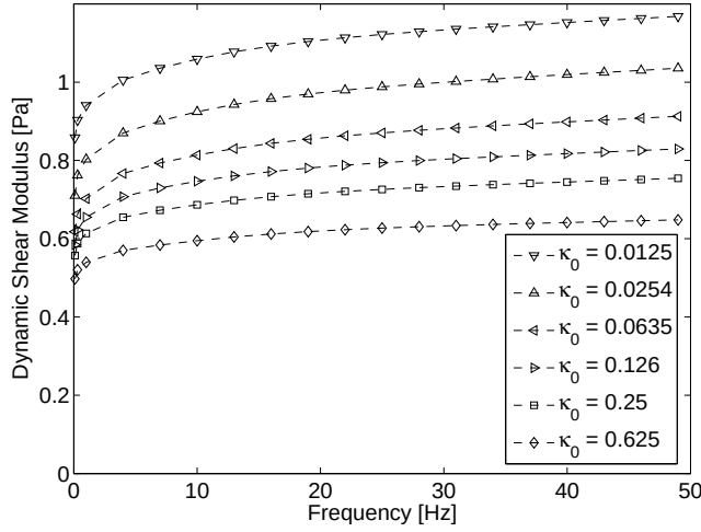
Figure 8: Simulated dynamic modulus using the equivalent time domain viscoelastic model.
