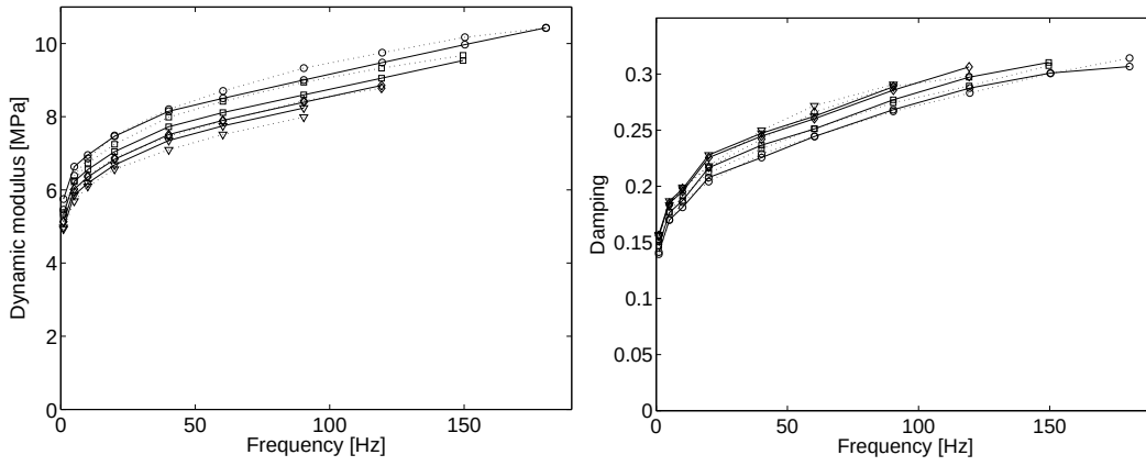
Figure 11: Dynamic shear modulus (left) and damping (right) of HGSD85. Solid line: material model. Dotted line: experimental data. \bigcirc : \kappa_0 = 1\% ; \nabla : \kappa_0 = 3\% ; \square : \kappa_0 = 7\% ; \triangle : \kappa_0 = 12\% .
