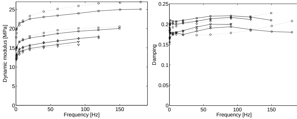
Figure 14: Dynamic shear modulus (left) and damping (right) of EPDM. Solid line: material model. Dotted line: experimental data. \bigcirc : \kappa_0 = 0.667\% ; \nabla : \kappa_0 = 2\% ; \square : \kappa_0 = 4\% ; \triangle : \kappa_0 = 6.7\% .
