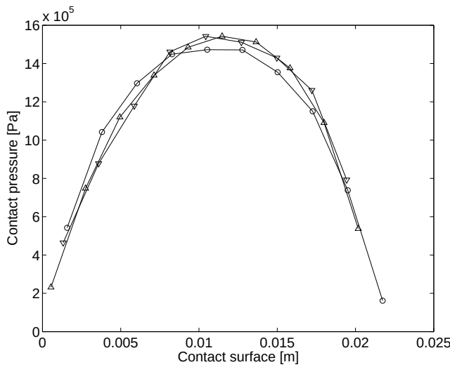
Figure 10: Contact pressure when rolling over a flat surface using fictive material models. ○: Elastic model; ▽: Elastoplastic model; △: Viscoelastic model.
