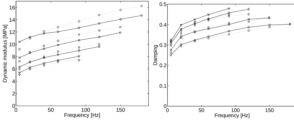
Figure 12: Dynamic shear modulus (left) and damping (right) of HNBR. Solid line: material model. Dotted line: experimental data. \bigcirc : \kappa_0 = 1\% ; \nabla : \kappa_0 = 3\% ; \square : \kappa_0 = 7\% ; \triangle : \kappa_0 = 12\% .
