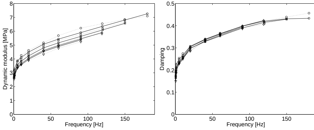
Figure 13: Dynamic shear modulus (left) and damping (right) of Hypalon72. Solid line: material model. Dotted line: experimental data. \bigcirc : \kappa_0 = 1\% ; \nabla : \kappa_0 = 3\% ; \square : \kappa_0 = 7\% ; \triangle : \kappa_0 = 12\% .
