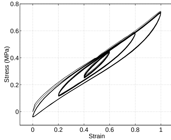
Figure 3: Hysteretic response, obtained from a double shear specimen subjected to a sinusoidal load at f = 0.05Hz .
