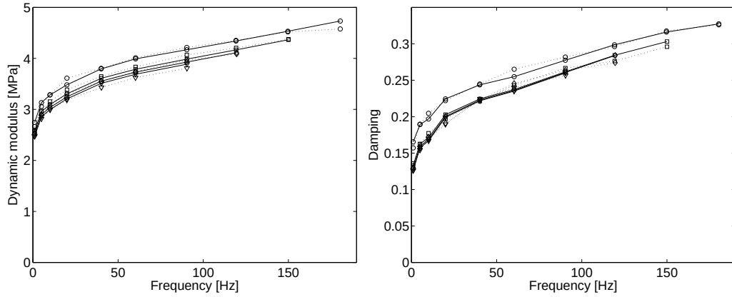
Figure 10: Dynamic shear modulus (left) and damping (right) of HGSD78. Solid line: material model. Dotted line: experimental data. \bigcirc : \kappa_0 = 1\% ; \nabla : \kappa_0 = 3\% ; \square : \kappa_0 = 7\% ; \triangle : \kappa_0 = 12\% .
