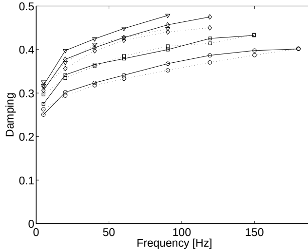
Figure 3: Damping of HNBR rubber. Solid line: elastoplastic-viscoelastic model. Dotted line: experimental data. \bigcirc : \kappa_0 = 1\% ; \square : \kappa_0 = 3\% ; \diamond : \kappa_0 = 7\% ; \nabla : \kappa_0 = 12\% .
