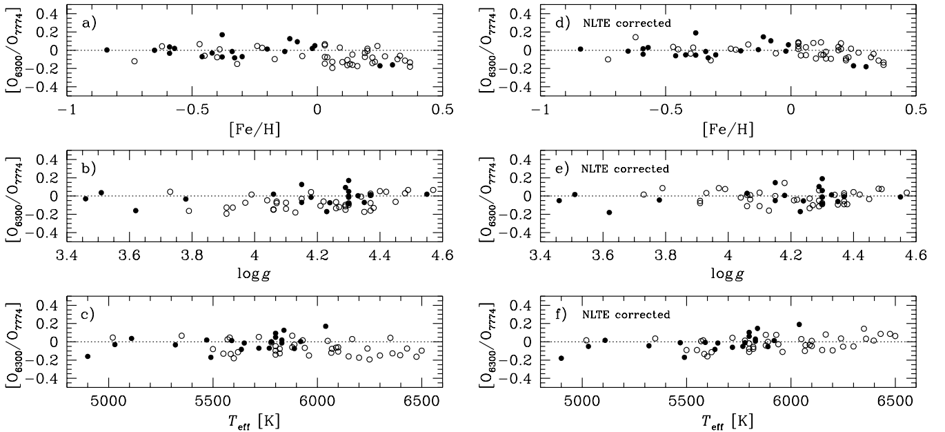
Fig. 8. a)–c) Difference between the oxygen abundances from the [\text{O I}]_{6300} line and the O I triplet at 7774 Å versus [\text{Fe}/\text{H}] , \log g , and T_{\text{eff}} . No NLTE corrections have been applied to the abundances from the triplet. d)–f) Difference between the oxygen abundances from the [\text{O I}]_{6300} line and the NLTE corrected abundances (according to the prescription in Gratton et al. 1999) from the O I triplet at 7774 Å versus [\text{Fe}/\text{H}] , \log g , and T_{\text{eff}} . Thin and thick disk stars are marked by open and filled circles, respectively.
