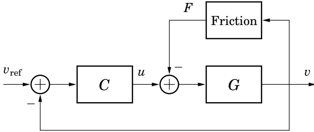
Figure 8. Velocity control system with Coulomb friction.
