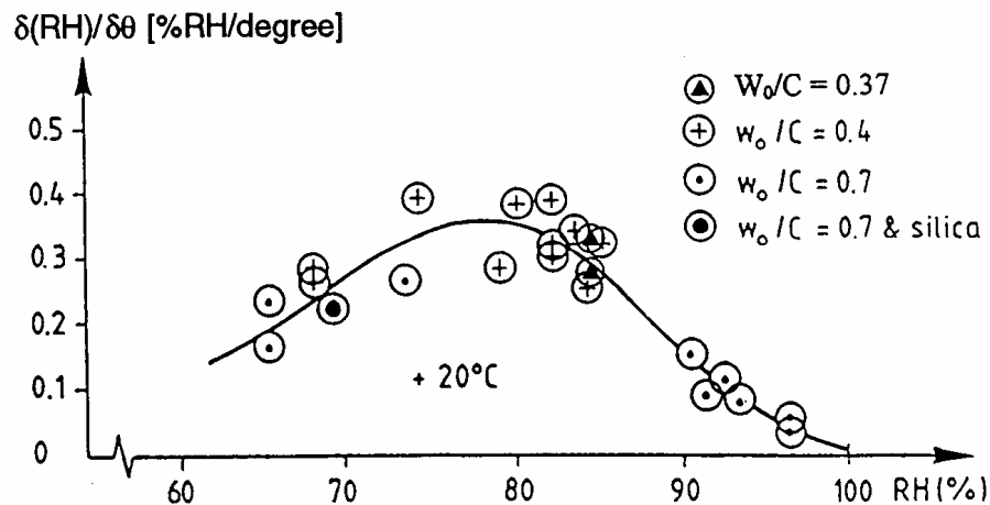
Figure 7: Change in RH for a certain change in temperature, assuming the total internal moisture content being constant. The average temperature is +22^\circ\text{C} . The figure expresses the influence of temperature on the equilibrium moisture curves (sorption isotherms) The curve is taken from /6/.
