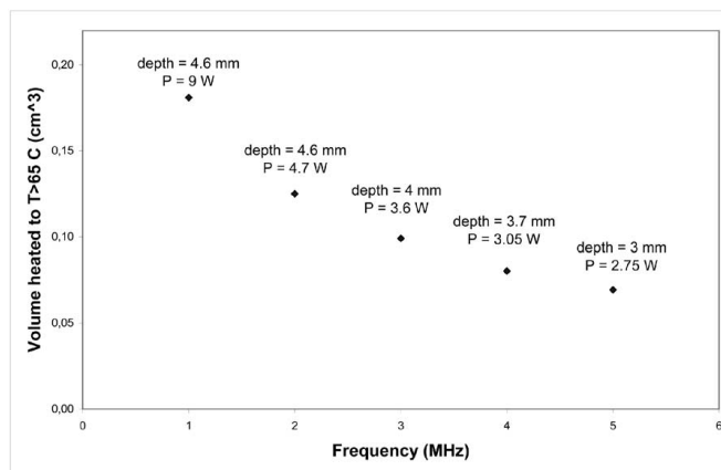
Fig. 5. The volume heated above 65°C vs. frequency with peak temperatures limited to 95°C after 120 s of US exposure. The depth at which the peak temperatures occur and the acoustic power used are also shown.
