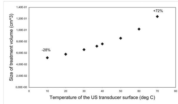
Fig. 10. The size of the treatment volume after 60 s of US exposure vs. temperature on the surface of the US transducer.
