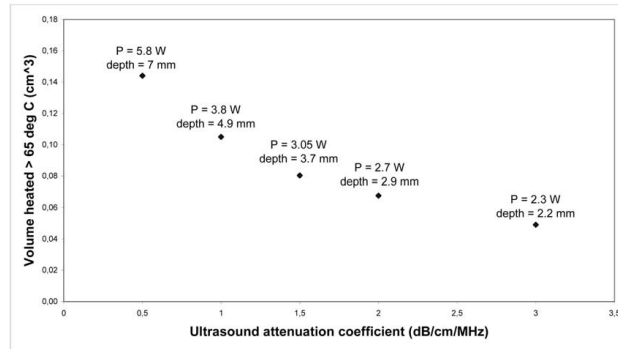
Fig. 8. The size of the treated volume as a function of the attenuation coefficient. The simulations were made for 120 s of 4-MHz US exposure with a peak temperature of 95°C.
