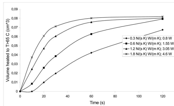
Fig. 7. The influence of the heat conductivity ( \lambda ) on the rate of treated volume change. The frequency was 4 MHz and the maximum temperature was limited to 95°C.
