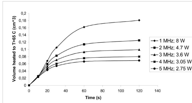
Fig. 6. The size of the treated volume vs. time for different frequencies, when the US intensity was limited to produce a peak temperature of 95°C. Lower frequencies result in larger treatment volumes.
