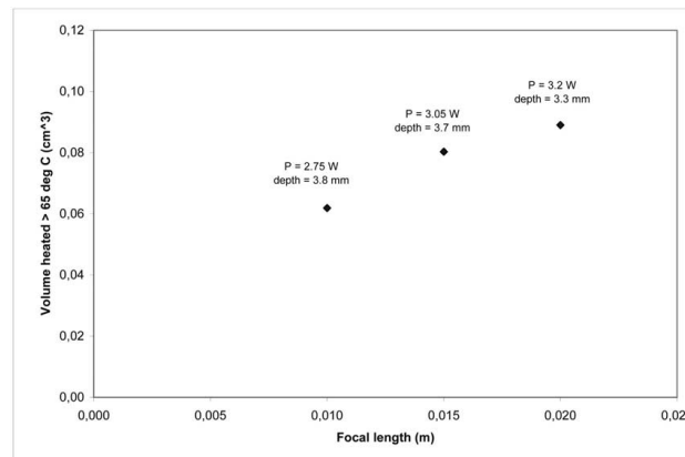
Fig. 9. The size of the treated volume after 120 s of 4-MHz US exposure as a function of the focal length, when the maximum temperature was limited to 95°C.
