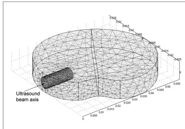
Fig. 1. The geometry and mesh used in the finite element simulations. The disk height used was 10 mm. The mesh is finer in the region of the US intensity field. The scale on the axis is in meters.
