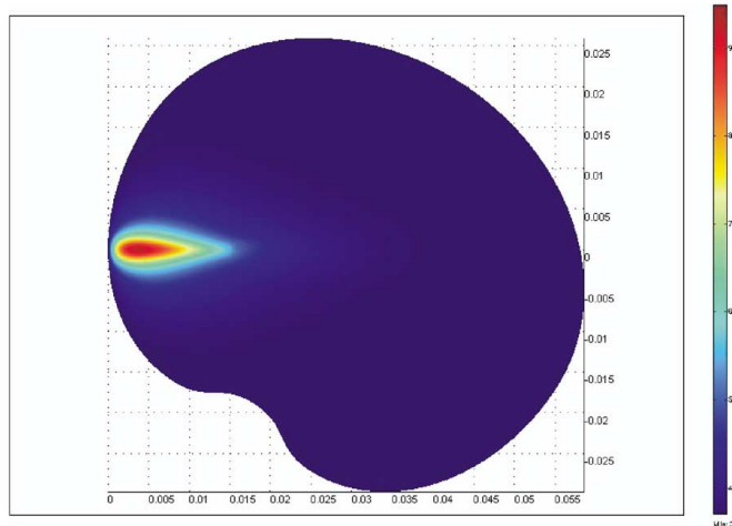
Fig. 3. The temperature distribution produced by the acoustic field shown in Fig. 2 after 120 s of US exposure. The units are in meters and in the scale at the right in ^{\circ}\text{C} . The length of the treatment volume is 12 mm and the width 4 mm for this simulation.
