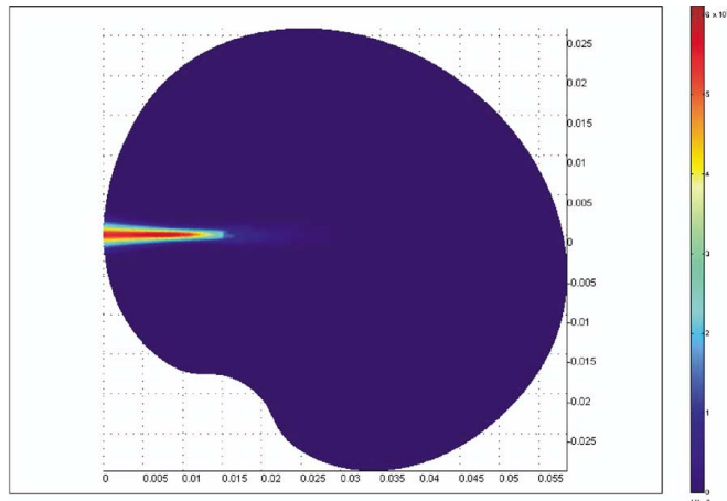
Fig. 2. A cross-section through the symmetry axis of the US beam that shows the applied intensity distribution in a disk with the properties shown in Table 1. The frequency used was 4 MHz and the acoustic power was 3.1 W. The unit of the color scale is in \text{W}/\text{m}^2 . The maximum intensity occurs at a depth of 8.7 mm and the half-maximum intensity width is 1.2 mm.
