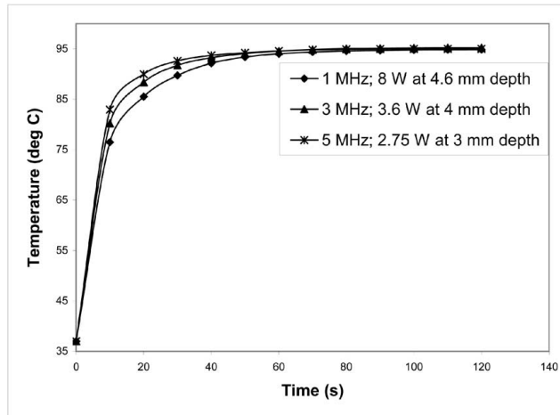
Fig. 4. Temperature as a function of time is shown in the point of maximum temperature for frequencies in the range of 1 to 5 MHz. The intensity was limited so that the peak temperature did not exceed 95°C.
