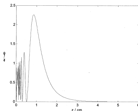
Fig. 7. The intensity distance-dependence of a transducer where a = 0.25 cm; A = 1 cm; f = 3.9 MHz; and \alpha = 0.5 \text{ dB cm}^{-1} \text{ MHz}^{-1} . The intensity peak, 2.3 I_0 , was obtained at 0.86 cm from the transducer.
