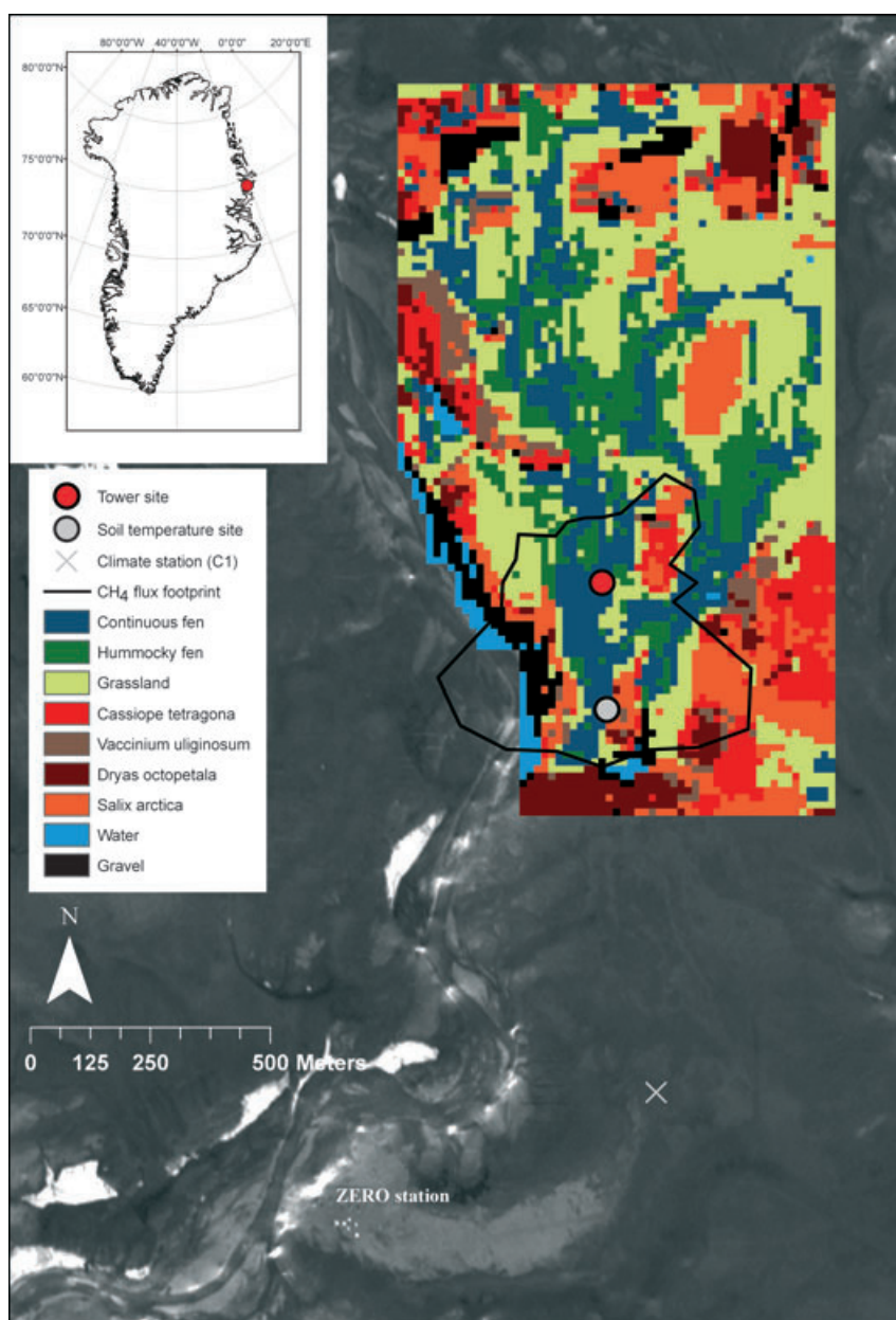
Fig. 1 The Zackenberg valley and the investigation area surrounding the Zackenberg research station (ZERO). A field-inventory map of the dominant plant communities observed in Rylekærene in July 2007 (Tagesson, 2011) is put on top of an IKONOS satellite image from 23 July 2000. The red mark on the Greenland map is the location of Zackenberg.
