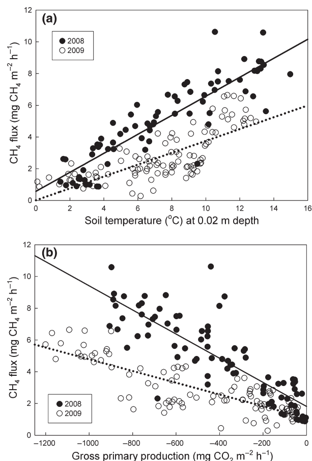
Fig. 5 (a) Daily average CH 4 fluxes against soil temperature at 0.02 m depth ( T_{0.02} ) and (b) against gross primary production (GPP) for the growing seasons 2008 and 2009. The solid lines are regressions for the 2008 data series, and the dotted lines are regressions for the 2009 data series (2008: CH 4 flux = 0.60 \times T_{0.02} + 0.57 , R^2 = 0.79 , n = 73 ; 2009: CH 4 flux = 0.37 \times T_{0.02} + 0.01 , R^2 = 0.55 , n = 98 ), (2008: CH 4 flux = -0.007 \times \text{GPP} + 1.90 , R^2 = 0.72 , n = 73 ; 2009: CH 4 flux = -0.004 \times \text{GPP} + 1.08 , R^2 = 0.66 , n = 98 ).
