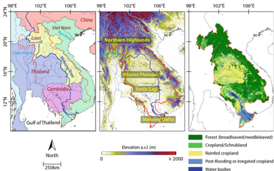
Fig. 17.1 Overview of the geography of the Lower Mekong Basin, shown with a red outline in the three maps. Left: the flow of the Mekong River through the basin. Middle: topography and the LMB’s major sub-basins. Right: land cover according to the GlobCover 2009 dataset (Bicheron et al. 2008)
