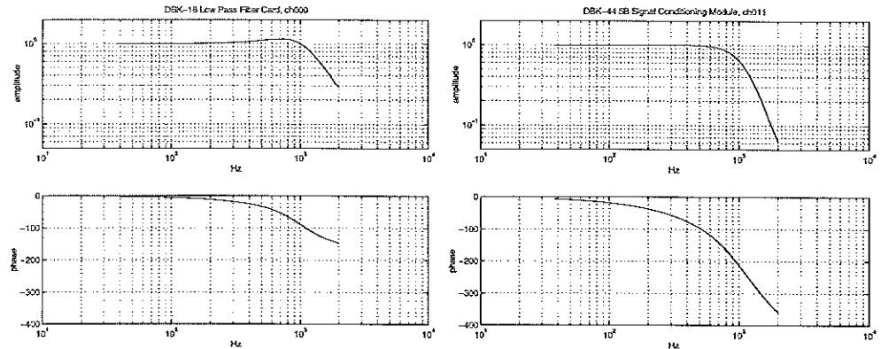
Figure 4 The Bode plots from the anti-aliasing filter (left) and the insulation unit (right). Both are low pass filtering with a bandwidth around 1 kHz.
