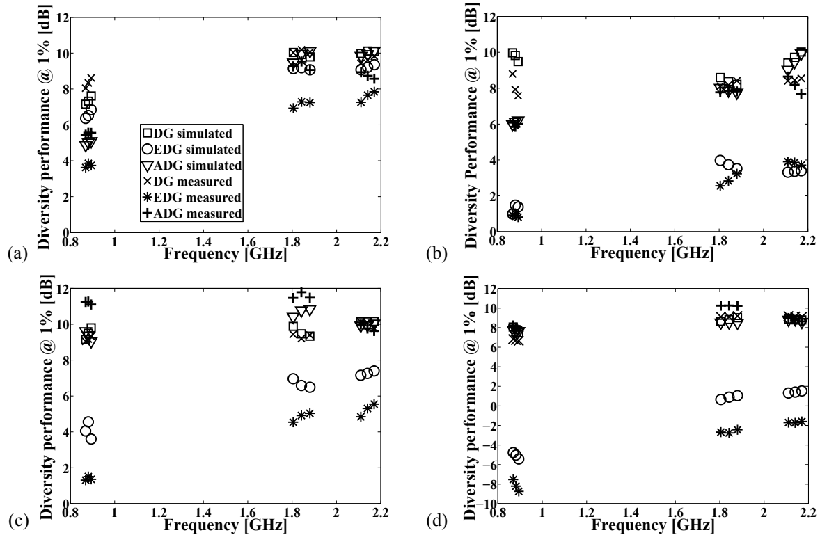
Fig. 11. Simulated and measured diversity performance at the 1 % probability level for the four user interaction scenarios: (a) freespace, (b) handheld position, (c) head only position, and (d) hand and head position.
