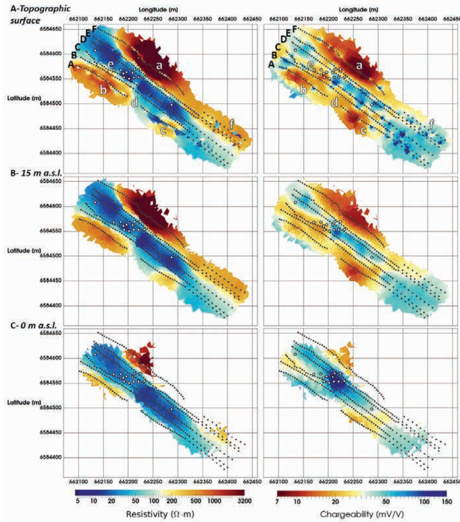
Figure 8 Inverted 3D model of electrical resistivity and integral chargeability plotted as 2D horizontal slices at (A) topographic surface, (B) 15 m a.s.l., and (C) 0 m a.s.l. Black dots are the electrode positions, and the black circles (white filled) show the position of geotechnical drillings; they are projected on the horizontal slices. Black uppercase labels mark the location of the six parallel lines (Figure 1). White lowercase labels highlight the presence of features that are discussed in the Results and Discussion section. Coordinate system Sweref 99 TM.
