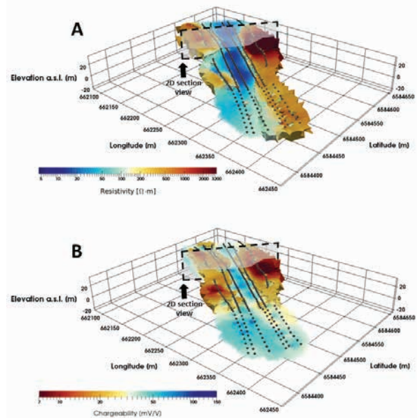
Figure 6 Inverted 3D model of (A) electrical resistivity and (B) integral chargeability. The surface electrical values are plotted, with a shading of the low resistivity and high chargeability values. Black dots mark the electrode positions. The 2D vertical section plane in Figure 9 is shown together with the point of view. Coordinate system Sweref 99 TM.
