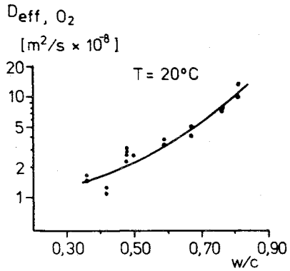
FIG 30 Measured effective diffusion coefficient for O_2 as a function of W/C. Cement type was Slite Portland cement. 2 The measurement was carried out at 20^\circ\text{C} and 50% RH. Specimen age approximately 1 year.
