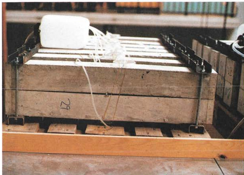
Photo 38. CO 2 initiation locally in crack by means of increased CO 2 content close to crack zone.
