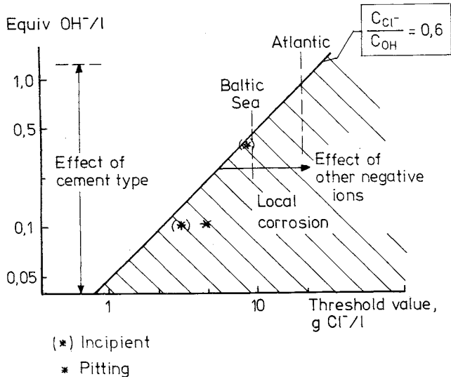
FIG 180. Threshold values.
