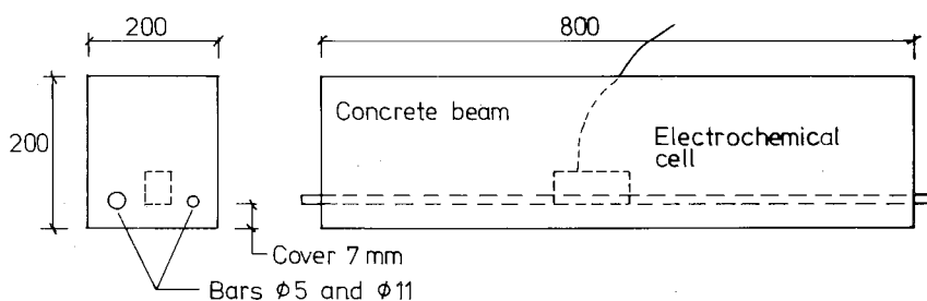
FIG 93. Placing of cells and reference bars in specimens.
