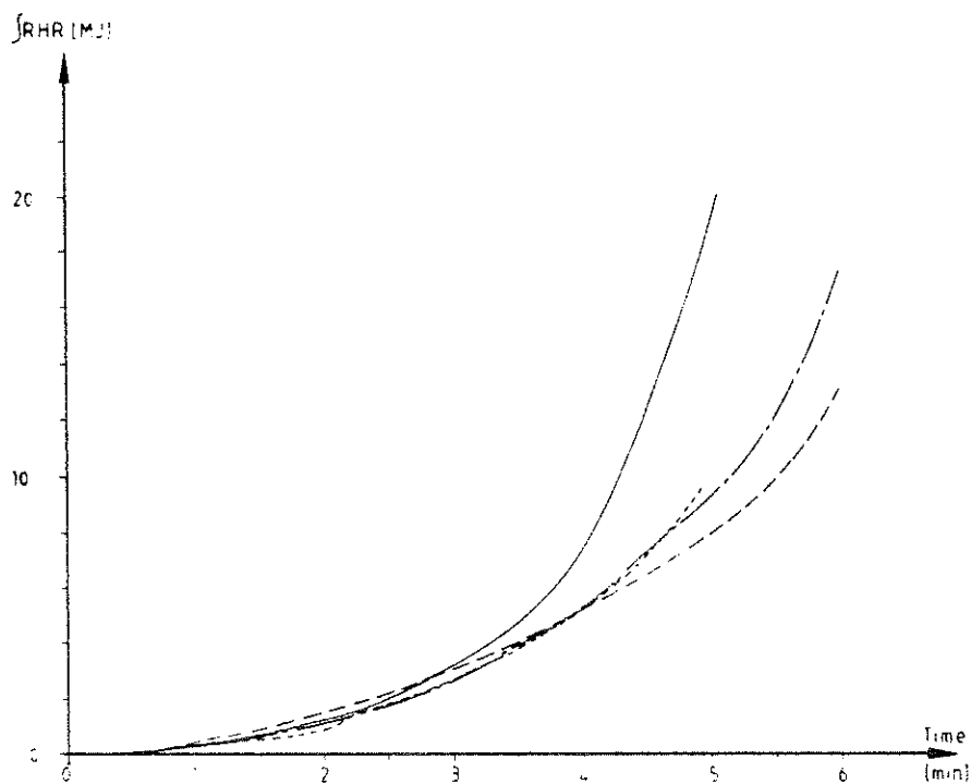
Figure D2b Total amount of heat released as a function of time for tests I:2 (medium density fibreboard) —, I:3 (particle board) ----, I:12 (wood panel, spruce) — — — and I:13 (paper wallcovering on particle board) — - —.
