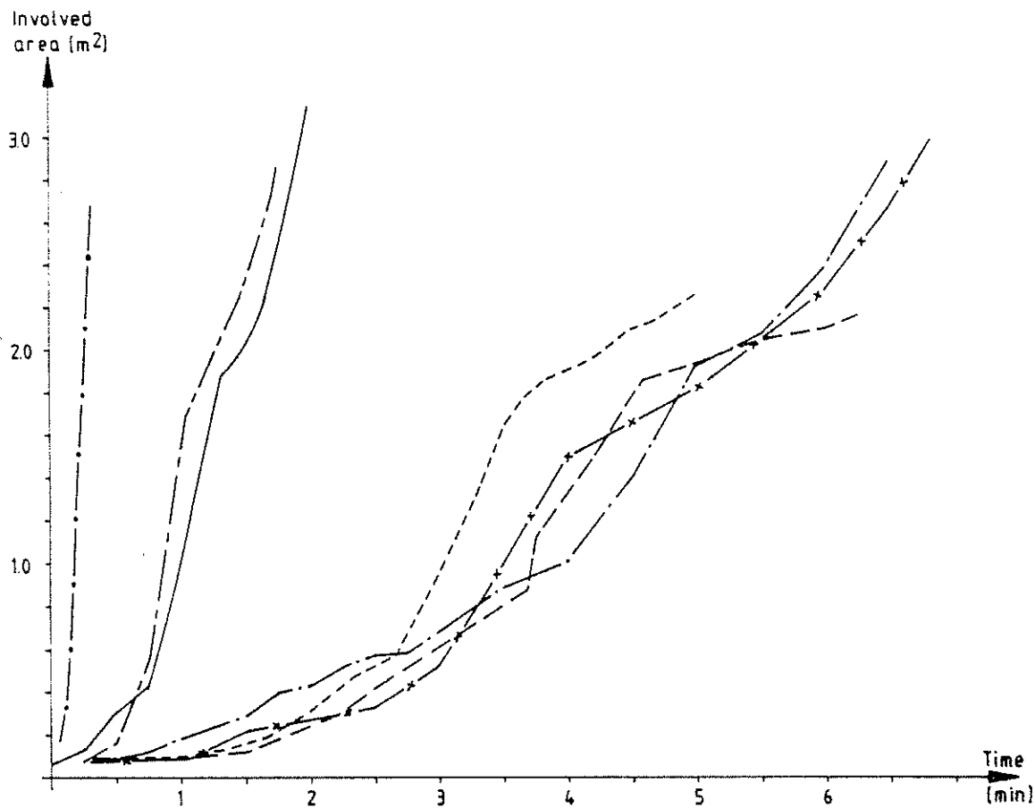
Figure G1 Area involved in flaming combustion as a function of time for tests I:1 (insulating fibreboard) —, I:2 (medium density fibreboard) ----, I:3 (particle board) — — —, I:8 (textile wallcovering on mineral wool) — - —, I:11 (rigid polyurethane foam) — o —, I:12 (wood panel, spruce) -·- and I:13 (paper wallcovering on particle board) —x—.
