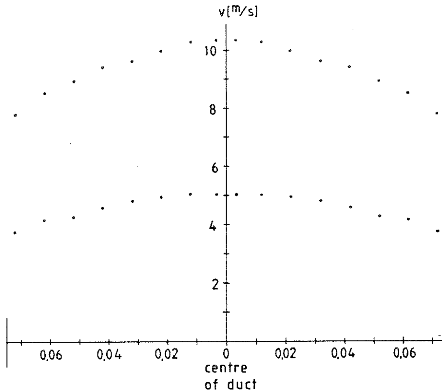
Figure 10 The velocity distribution across the exhaust duct (diameter = 0.15 m). The measurements were made at two different velocities, \sim 5 m/s and \sim 10 m/s. (Dimensions are in m.)
