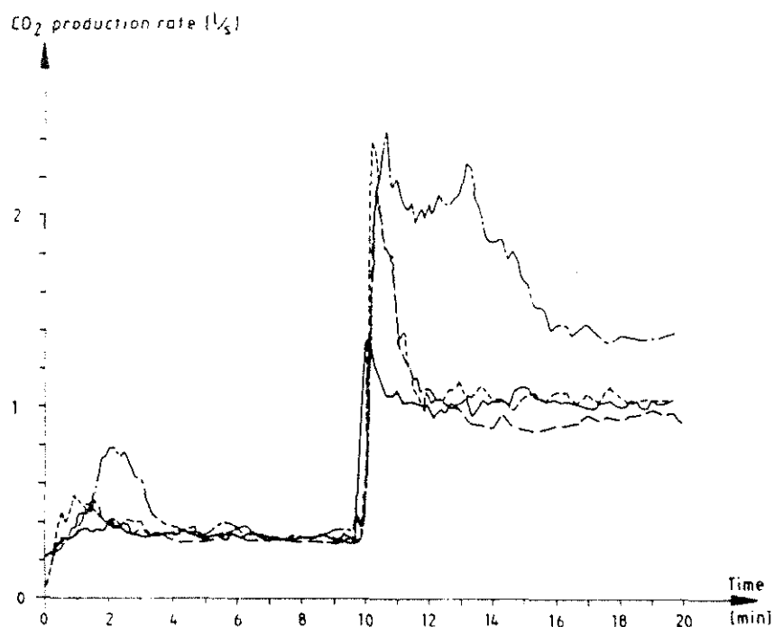
Figure E10a \text{CO}_2 production rate for tests I:4 (gypsum plaster board) —, I:5 (PVC wallcovering on gypsum plaster board) ----, I:6 (paper wallcovering on gypsum plaster board) — — — and I:7 (textile wallcovering on gypsum plaster board) — - —.
