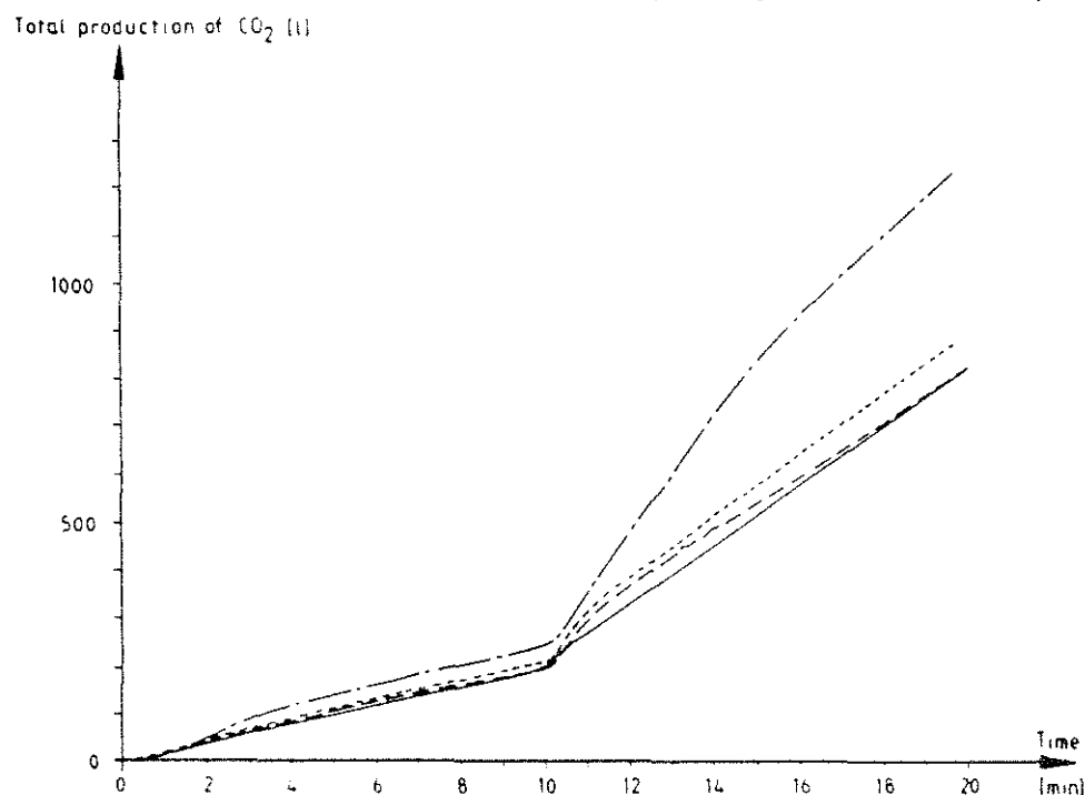
Figure E10b Total production of \text{CO}_2 as a function of time for tests I:4 (gypsum plaster board) —, I:5 (PVC wallcovering on gypsum plaster board) ----, I:6 (paper wallcovering on gypsum plaster board) — — — and I:7 (textile wallcovering on gypsum plaster board) — - —.
