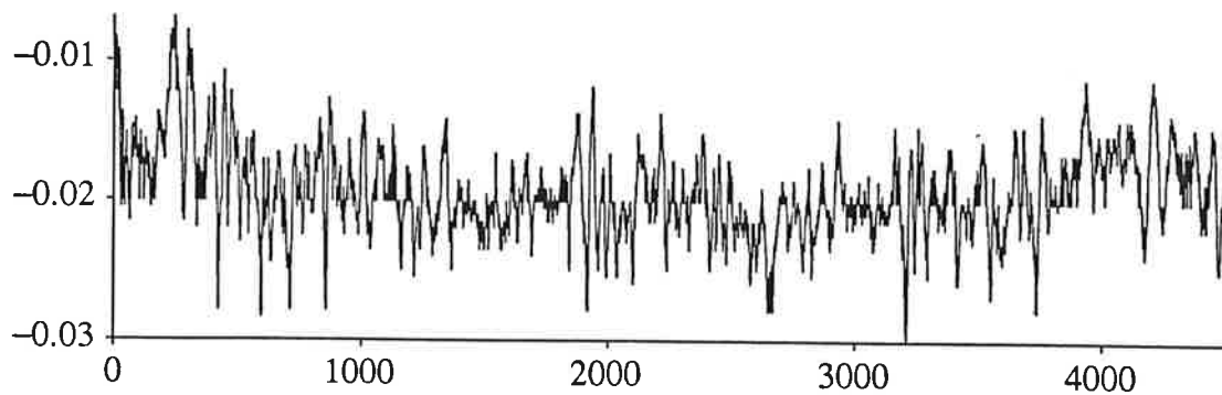
Figure 5. Experiment D : Sway ( 371.7 \text{ [Nm/scale unit]} ) in frontal plane ( yz ) vs. time. Time scale in units of 0.04 [s].
