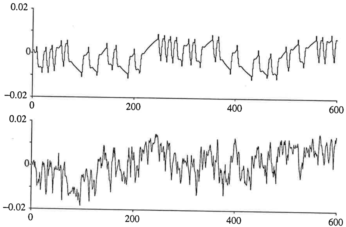
Figure 15. Sagittal sway of model with input of experiment D : Simulated output from third order estimated model ( upper ). Sagittal sway of experiment D : Real output ( lower ). Time scale in units of 0.2 [s].
