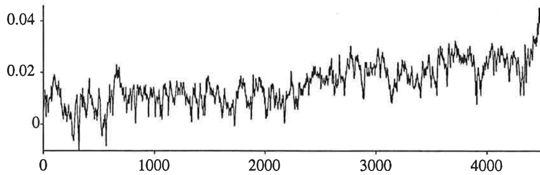
Figure 6. Experiment E : Sway (371.7 [ Nm/scale unit ]) in saggittal plane ( xz ) vs. time. Time scale in units of 0.04 [ s ].
