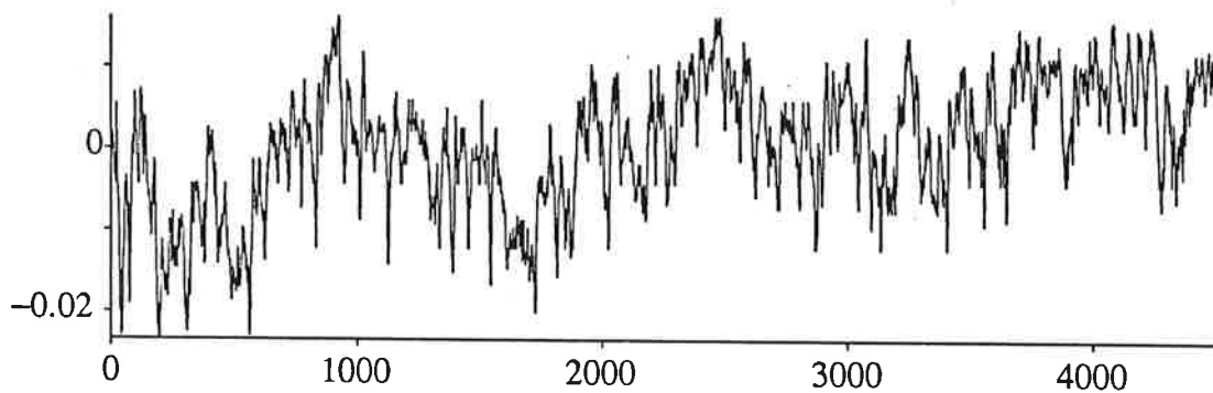
Figure 4. Experiment D : Sway ( 371.7 \text{ [Nm/scale unit]} ) in saggittal plane ( xz ) vs. time. Time scale in units of 0.04 [s].
