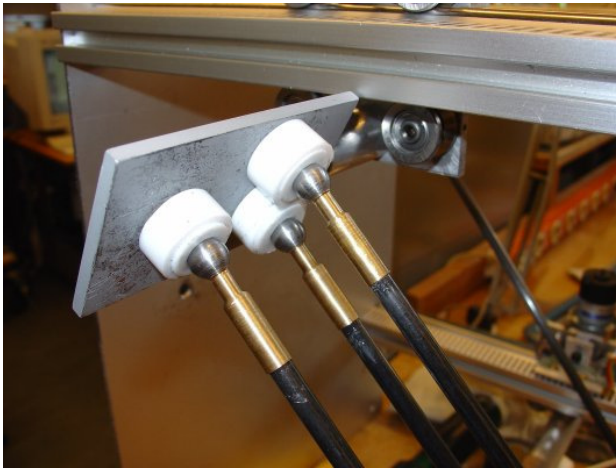
Figure 3.2 Magnetic spherical joints for easy reconfiguration of arm links for the table model of the Gantry-Tau parallel kinematic robot.
