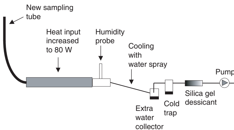
Figure 12. New design of water measuring instrument
