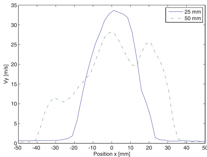
Figure 8 Velocity profile for hollow cone nozzle at 25 mm and 50 mm below nozzle
