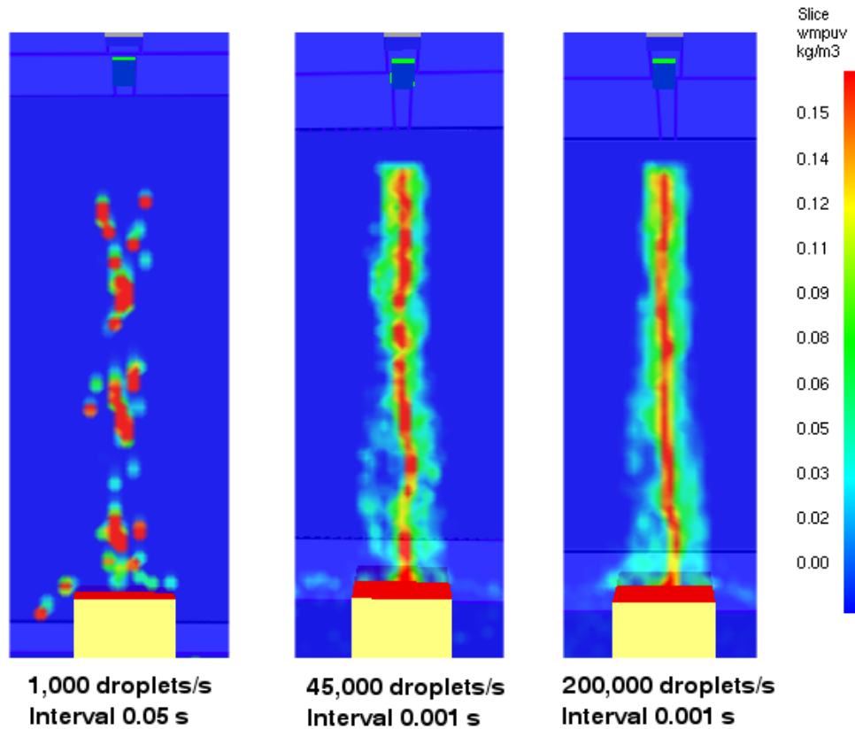
Figure 9. Simulation of water mist spray without fire on the coarse grid. The number of water droplets release per second have been varied and the colour indicates the water droplet concentration in \text{kg/m}^3 . (The default setup in FDS uses 1000 droplets pr. second released with an interval of 0.05 s, left picture)
