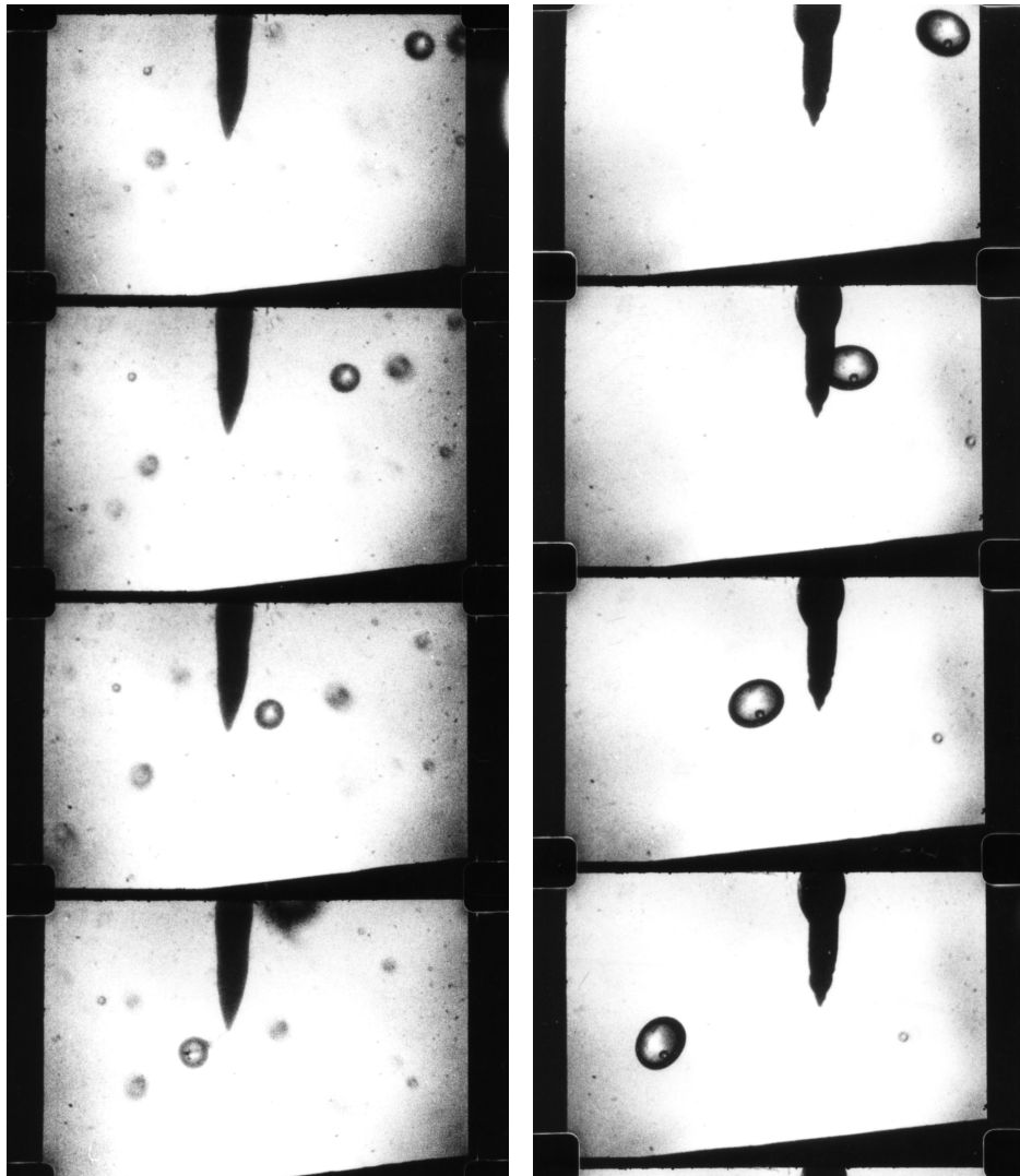
Figure 6. Measurement of size and speed with high speed camera, two different measurements. In the film on the left, droplet size is 400µm and in the film on the right, 800µm. From Nolan [40]
