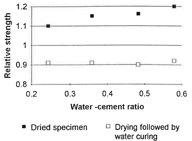
Fig. 6 - Strength with intensive drying of cores, f_{cd} , and strength with drying followed by water curing, f_{cw} .
