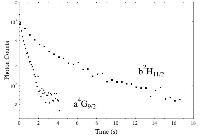
Fig. 1. Typical lifetime curves (after corrections) for the levels a^4G_{9/2} and b^2H_{11/2} .
