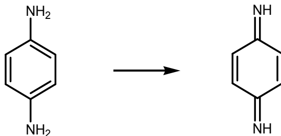
Figure 2. Transformation of p-phenylenediamine to quinonediimine by oxidation. p-Phenylenediamine is shown on the left and the oxidation product quinonediimine (p-benzoquinonediimine) is shown on the right. N, nitrogen; H, hydrogen.
