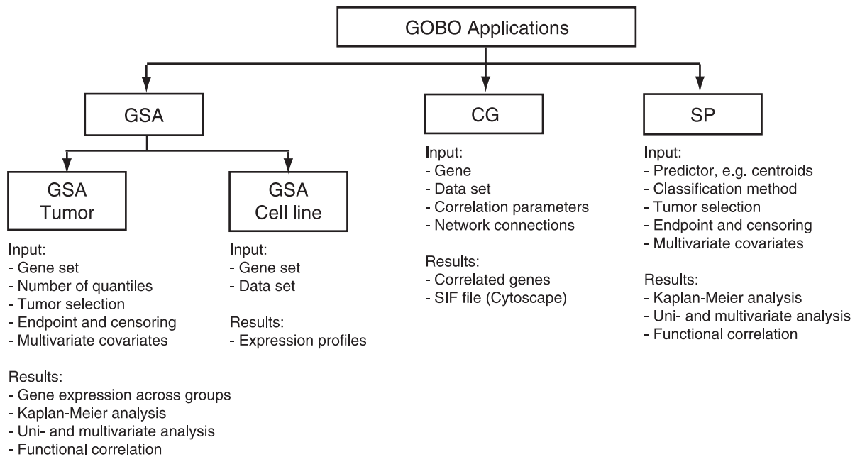
Figure 1. Architecture of GOBO. (A) Flowchart of the GOBO software illustrating the three different modules, data set module (black), web interface module (red) and analysis module (blue). (B) Layout of GOBO applications with respect to input and results generated. doi:10.1371/journal.pone.0017911.g001
