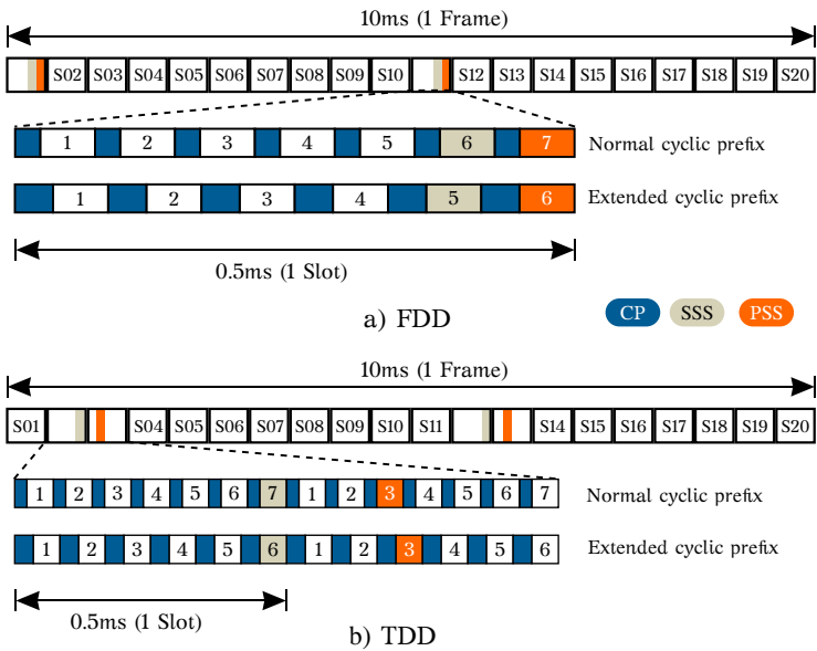
Figure 3.5.: Location of PSS and SSS in LTE for: a) FDD and b) TDD.
