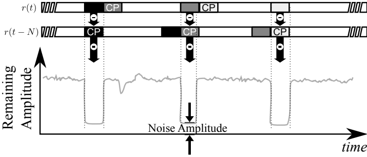
Figure 6.1.: Graphical representation subtraction |\Upsilon(n)| with channel h(n) = \delta(n) , \tau = 0 , and \Delta\varphi = 0 .
