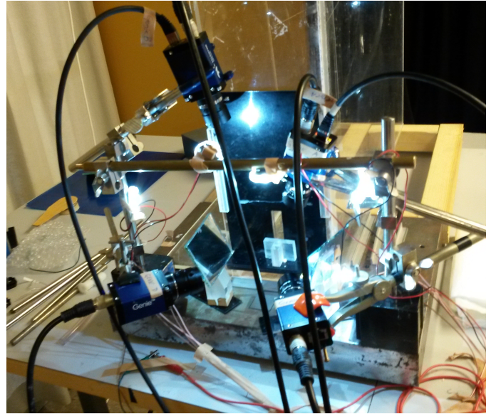
Fig. 1: The experimental setup with four cameras, lights and a calibration object.
